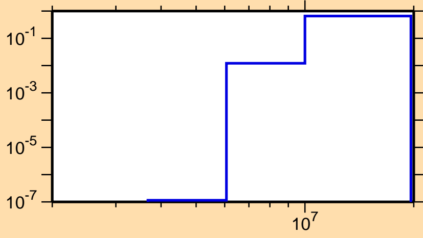
\sigma vs. E for ^{145}\text{Dy}(n,np)
