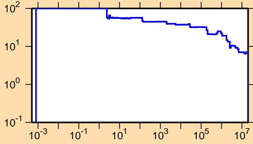
\Delta\sigma/\sigma vs. E for ^{146}\text{Dy}(n,\text{nonel.})
