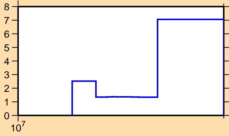
\Delta\sigma/\sigma vs. E for ^{146}\text{Dy}(n,\text{tot.})
