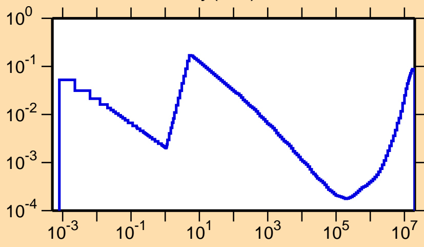
\sigma vs. E for ^{146}\text{Dy}(n,\alpha)
