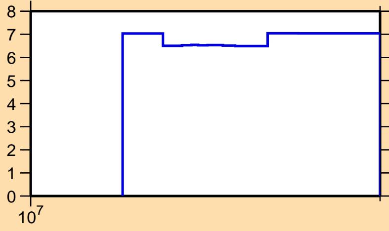
\Delta\sigma/\sigma vs. E for ^{146}\text{Dy}(n,\text{nonel.})
