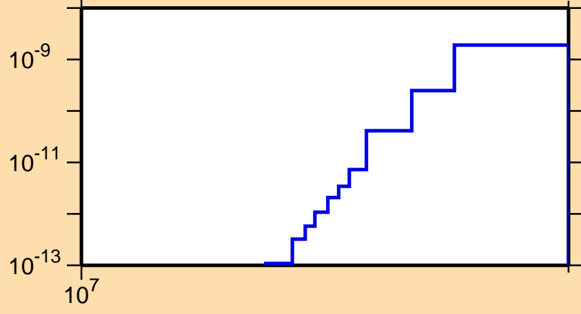
\sigma vs. E for ^{146}\text{Dy}(\text{mt117})
