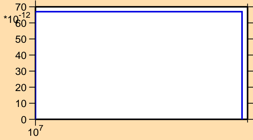
\sigma vs. E for ^{146}\text{Dy}(n,nd)
