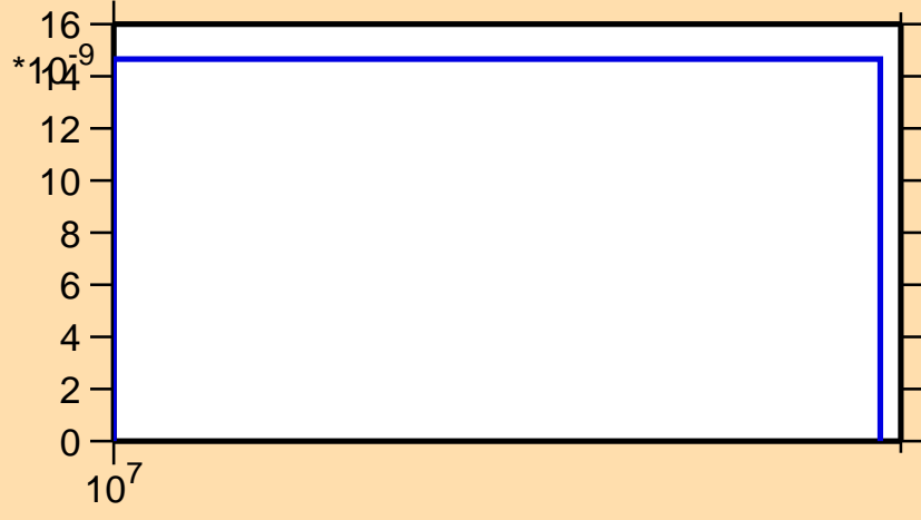
\sigma vs. E for ^{146}\text{Dy} (mt 45)
