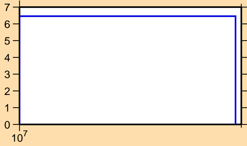
\Delta\sigma/\sigma vs. E for ^{146}\text{Dy}(n,\text{el.})
