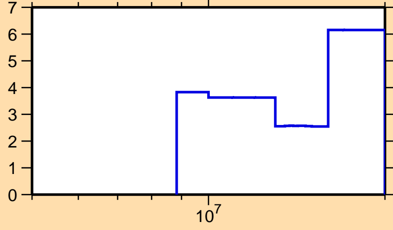
\Delta\sigma/\sigma vs. E for ^{147}\text{Dy}(n,\text{tot.})
