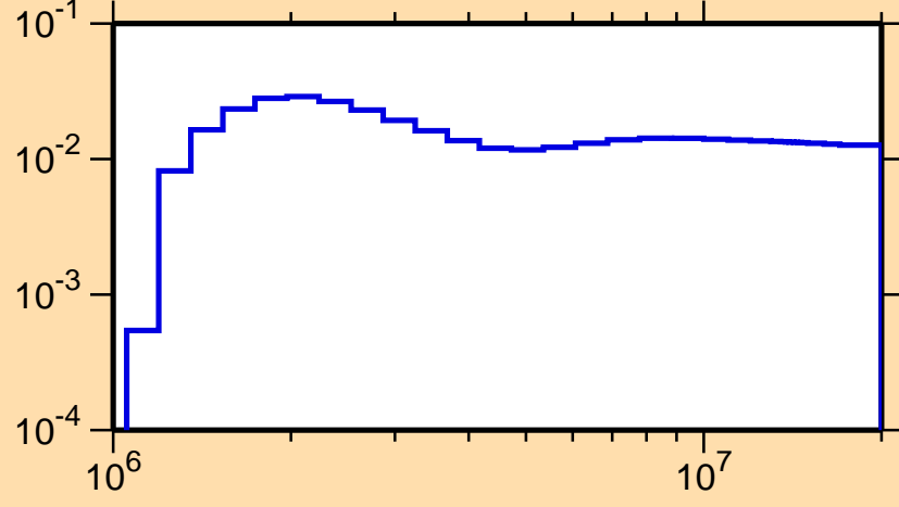
\sigma vs. E for ^{147}\text{Dy}(n,n_4)
