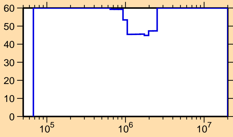
\Delta\sigma/\sigma vs. E for ^{147}\text{Dy}(n,n_1)
