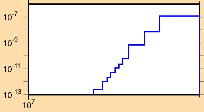
\sigma vs. E for ^{147}\text{Dy} (mt 45)
