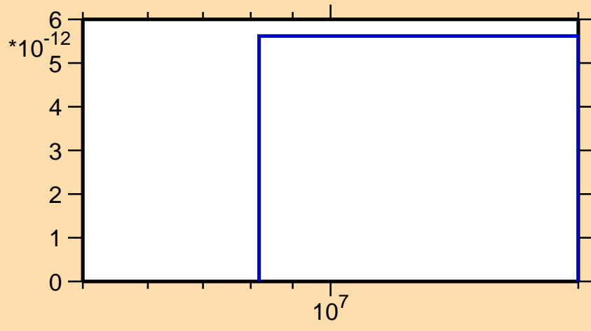
\sigma vs. E for ^{147}\text{Dy}(\text{mt117})
