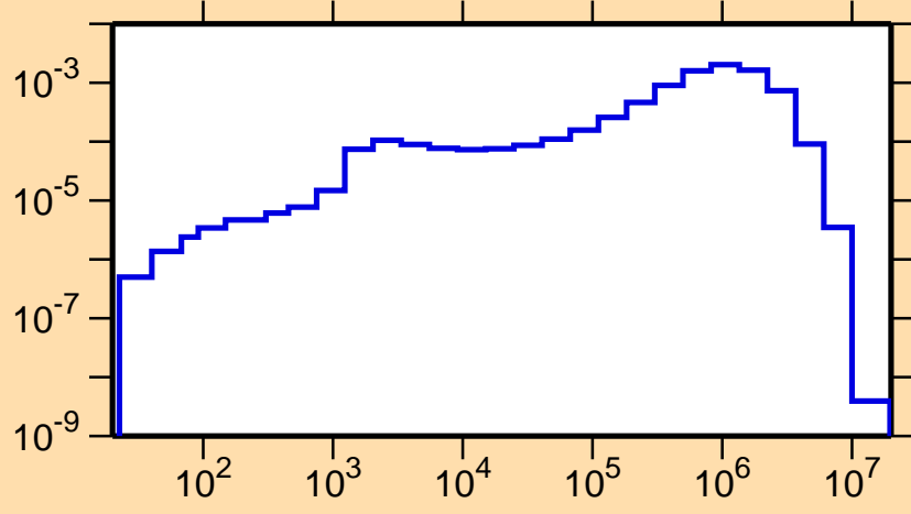
\sigma vs. E for ^{147}\text{Dy}(n,n_1)
