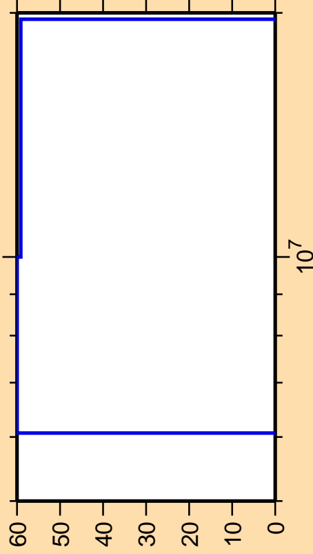
\Delta\sigma/\sigma vs. E for ^{147}\text{Dy}(n,2n)
