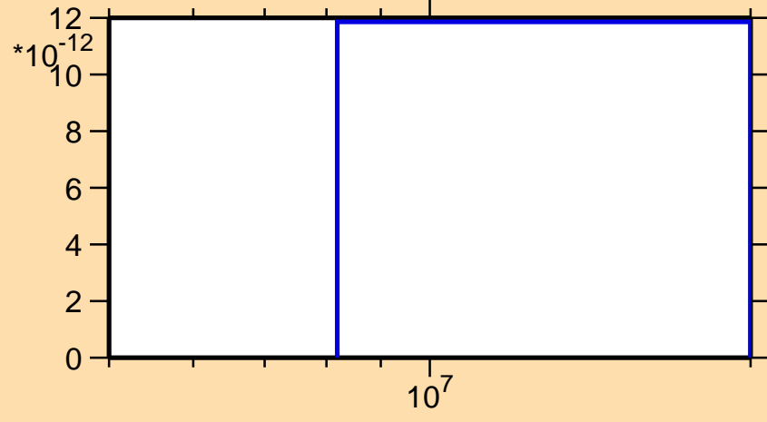
\sigma vs. E for ^{148}\text{Dy}(n,\text{pt})
