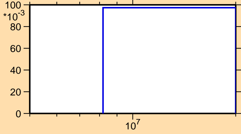
\sigma vs. E for ^{148}\text{Dy}(n,2n)
