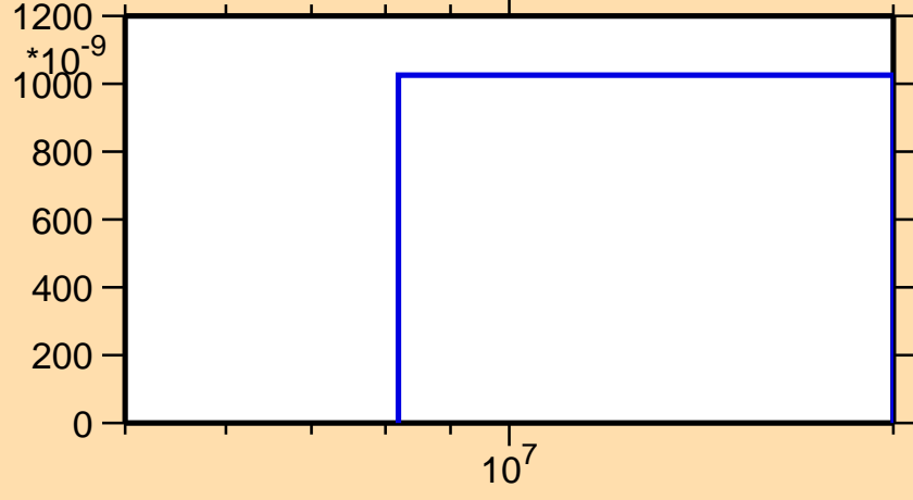
\sigma vs. E for ^{148}\text{Dy}(n,\text{pd})
