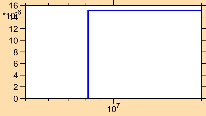
\sigma vs. E for ^{148}\text{Dy}(n,t)
