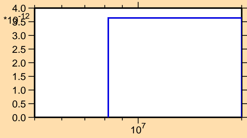
\sigma vs. E for ^{148}\text{Dy}(\text{mt117})
