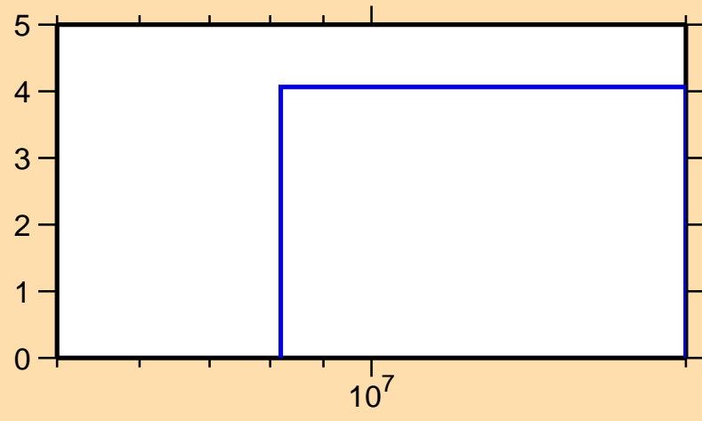
\Delta\sigma/\sigma vs. E for ^{148}\text{Dy}(n,\text{tot.})
