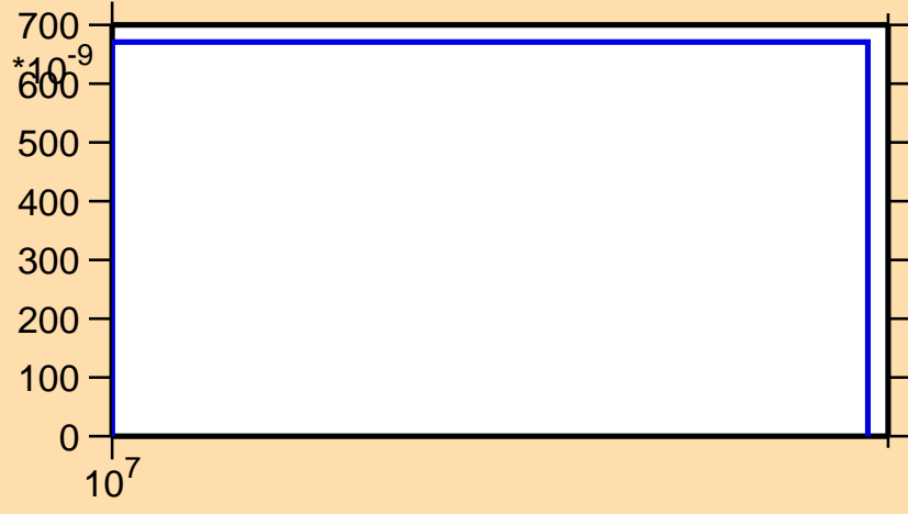
\sigma vs. E for ^{149}\text{Dy}(n,nd)
