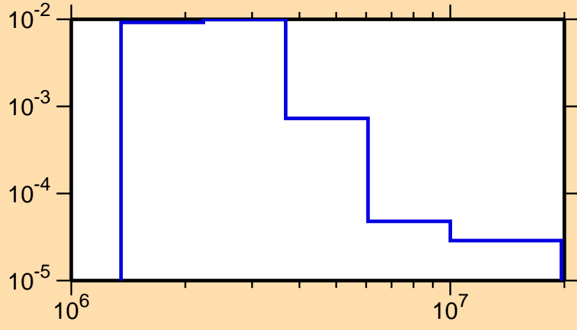
\sigma vs. E for ^{149}\text{Dy}(n,n_4)
