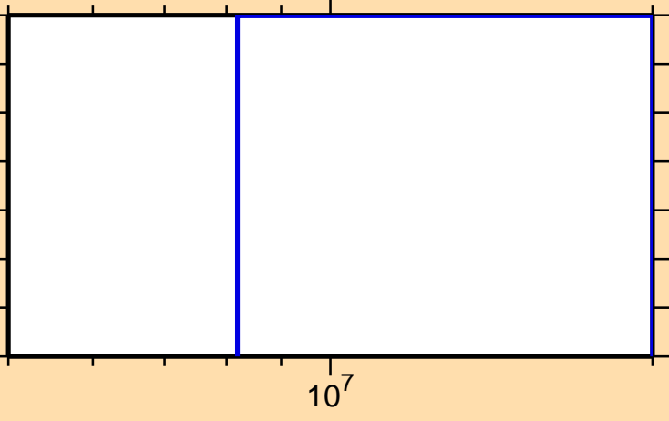
\sigma vs. E for ^{149}\text{Dy}(n,\text{pd})
