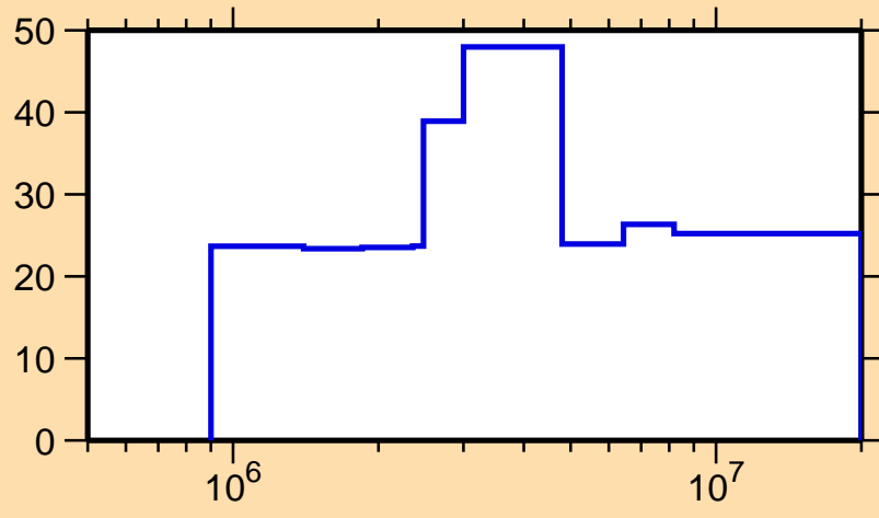
\Delta\sigma/\sigma vs. E for ^{149}\text{Dy}(n,n_1)
