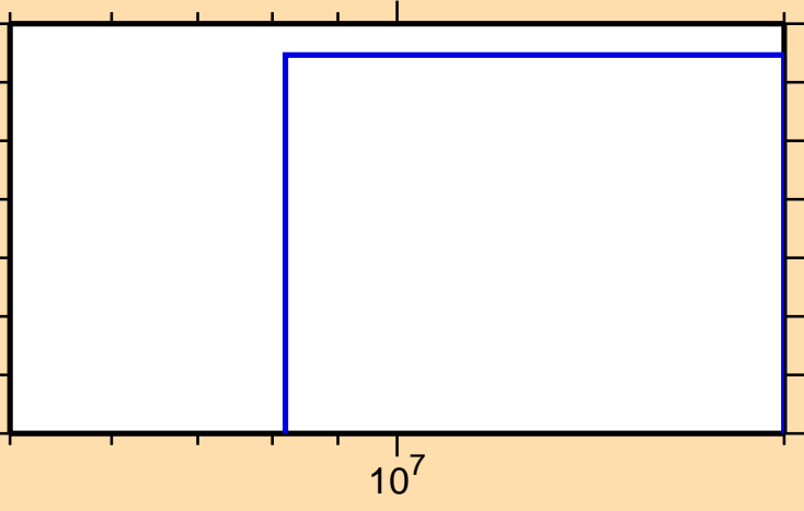
\sigma vs. E for ^{149}\text{Dy}(n,\text{pt})
