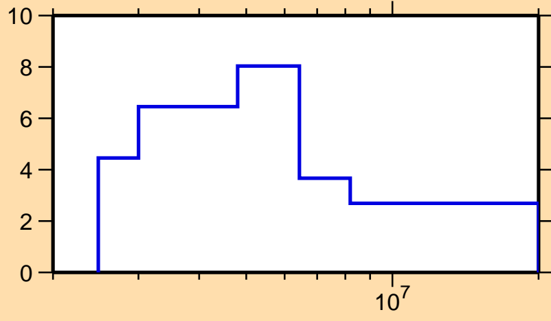
\Delta\sigma/\sigma vs. E for ^{149}\text{Dy}(n, tot.)
