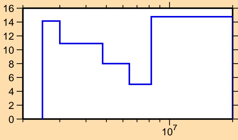
\Delta\sigma/\sigma vs. E for ^{149}\text{Dy}(n,n\text{cont.})
