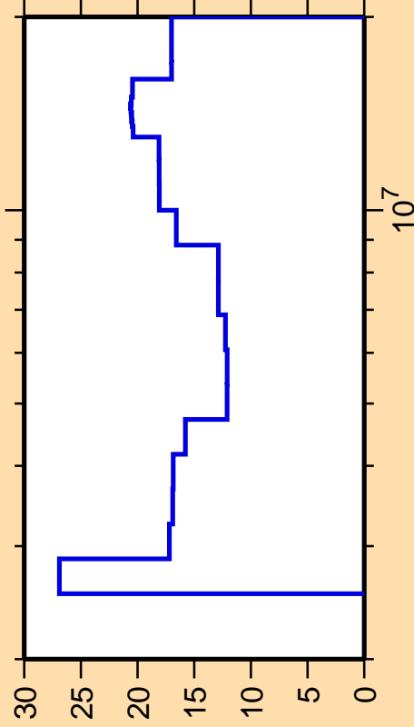
\Delta\sigma/\sigma vs. E for ^{150}\text{Dy}(n, ncont.)
