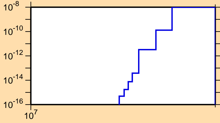
\sigma vs. E for ^{150}\text{Dy}(n,\text{pt})
