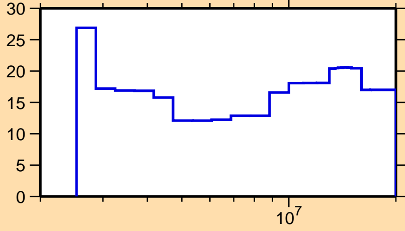
\Delta\sigma/\sigma vs. E for ^{150}\text{Dy}(n,n\text{cont.})
