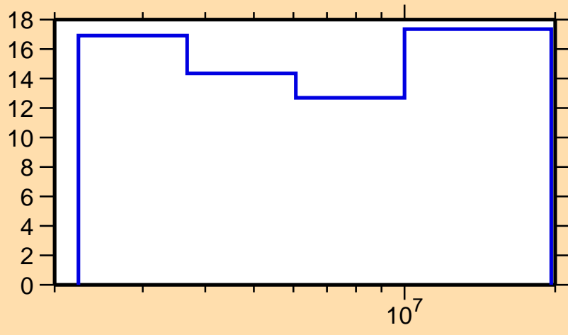
\Delta\sigma/\sigma vs. E for ^{150}\text{Dy}(n,n\text{cont.})
