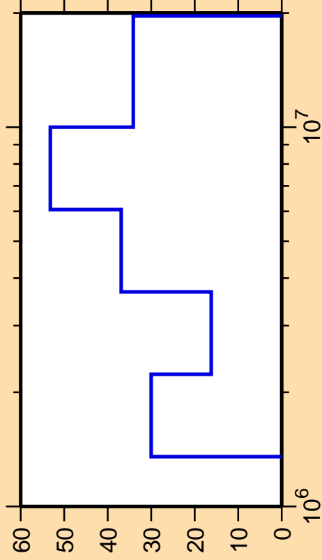
\Delta\sigma/\sigma vs. E for ^{150}\text{Dy}(n,n_3)
