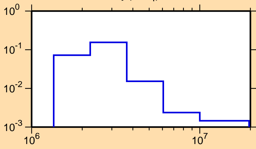
\sigma vs. E for ^{150}\text{Dy}(n,n_4)
