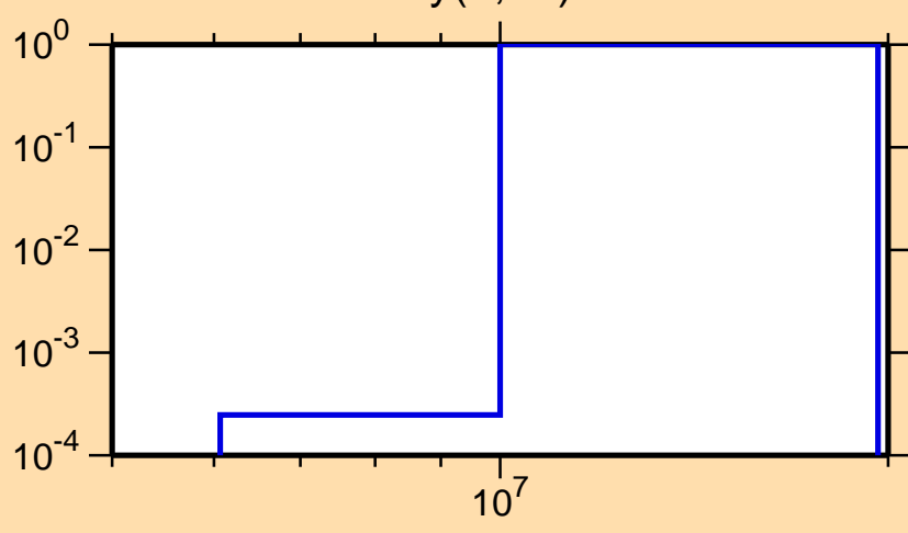
\sigma vs. E for ^{150}\text{Dy}(n,2n)
