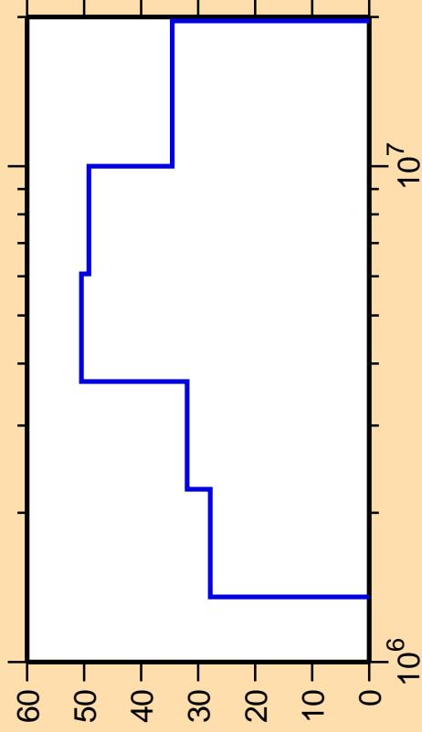
\Delta\sigma/\sigma vs. E for ^{150}\text{Dy}(n,n_4)
