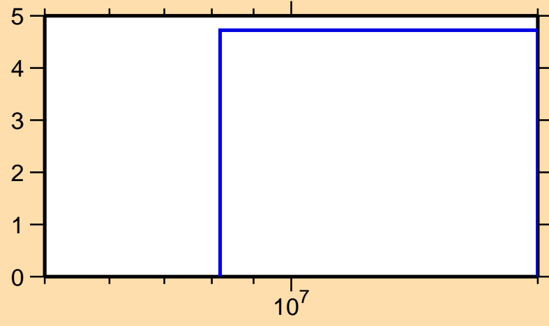
\Delta\sigma/\sigma vs. E for ^{150}\text{Dy}(n,\text{nonel.})
