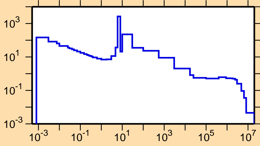
\sigma vs. E for ^{150}\text{Dy}(n,\gamma)
