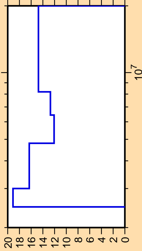
\Delta\sigma/\sigma vs. E for ^{150}\text{Dy}(n, ncont.)
