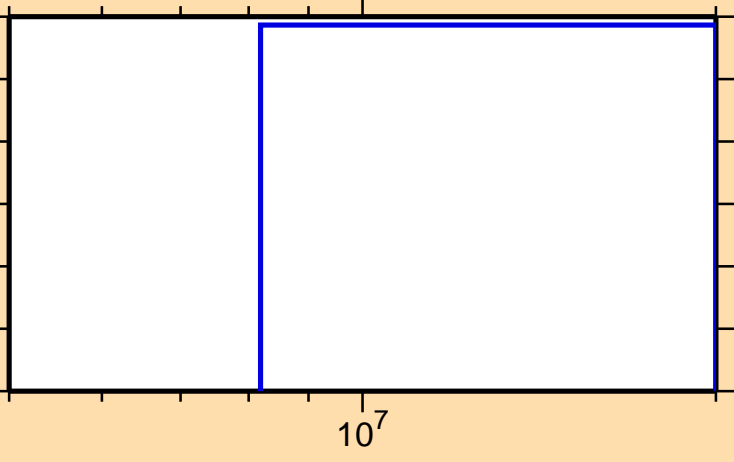
\sigma vs. E for ^{150}\text{Dy}(n,2n\alpha)
