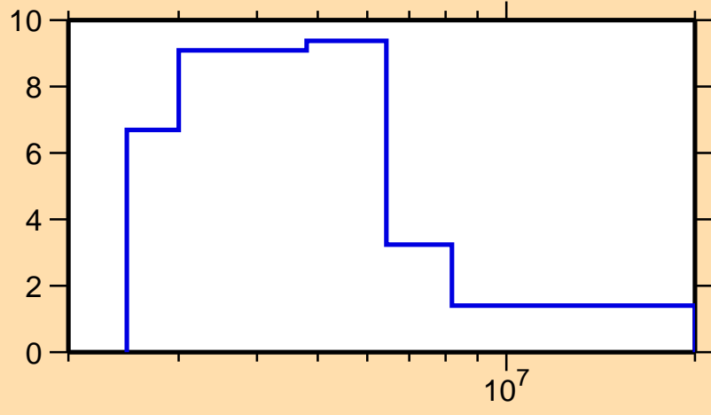
\Delta\sigma/\sigma vs. E for ^{150}\text{Dy}(n, tot.)
