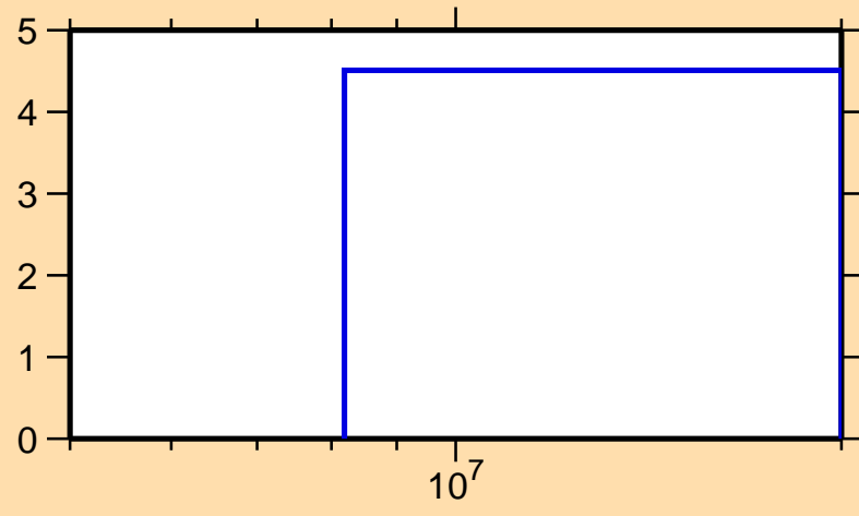
\Delta\sigma/\sigma vs. E for ^{150}\text{Dy}(n,\text{el.})
