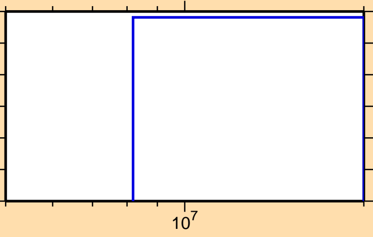
\sigma vs. E for ^{150}\text{Dy}(\text{mt117})
