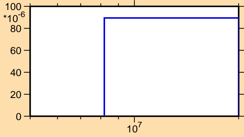
\sigma vs. E for ^{150}\text{Dy}(n,t)
