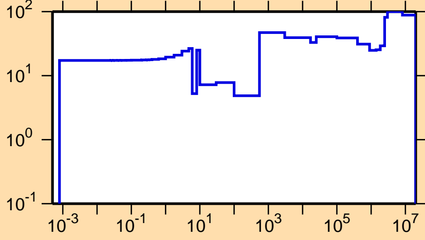
\Delta\sigma/\sigma vs. E for ^{150}\text{Dy}(n,\gamma)
