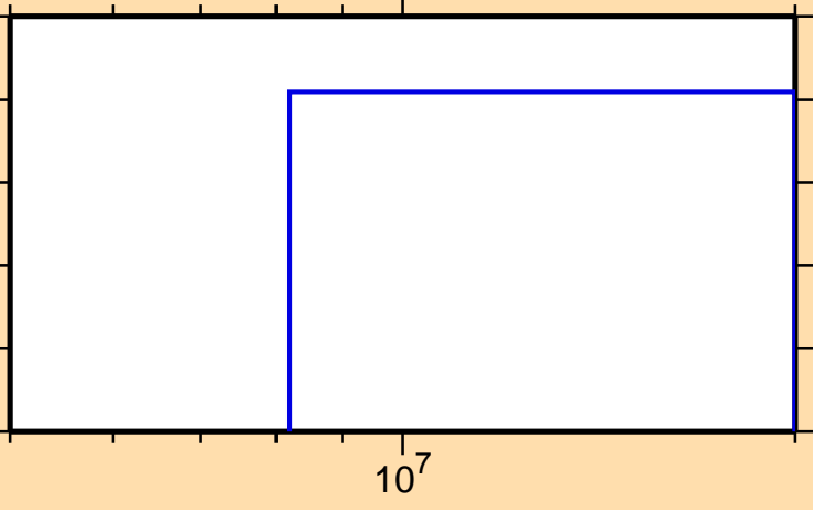
\sigma vs. E for ^{150}\text{Dy}(n,2np)
