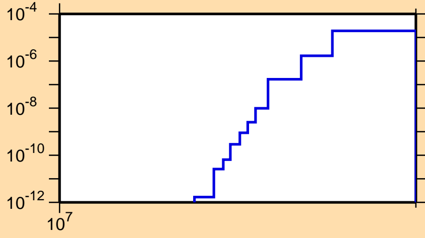
\sigma vs. E for ^{151}\text{Dy}(n,nd)
