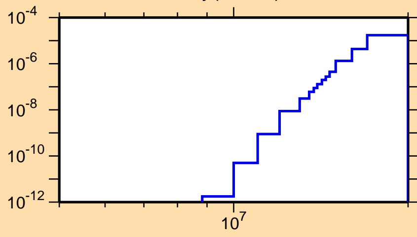
\sigma vs. E for ^{151}\text{Dy}(n,\text{He}3)
