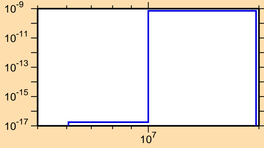
\sigma vs. E for ^{151}\text{Dy}(\text{mt117})
