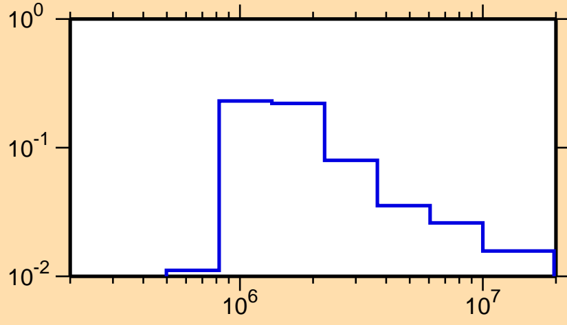
\sigma vs. E for ^{151}\text{Dy}(n,n_4)
