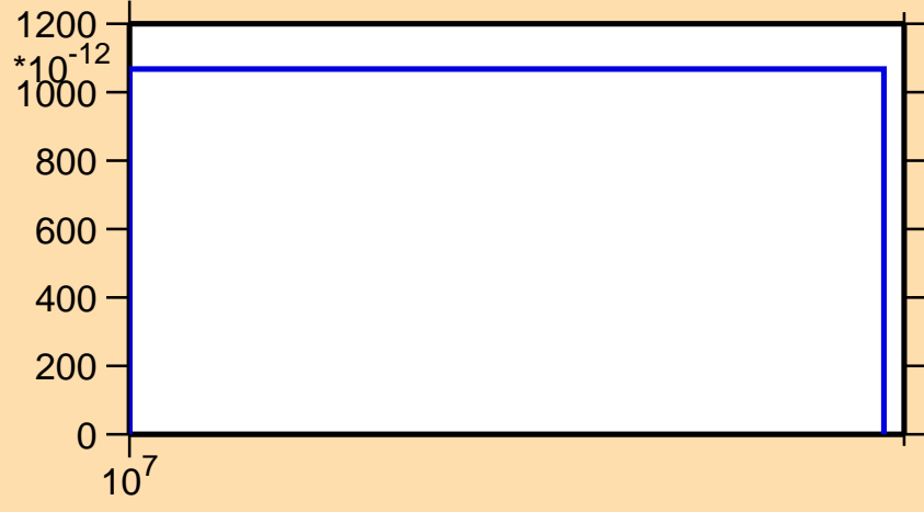
\sigma vs. E for ^{151}\text{Dy}(n,pt)
