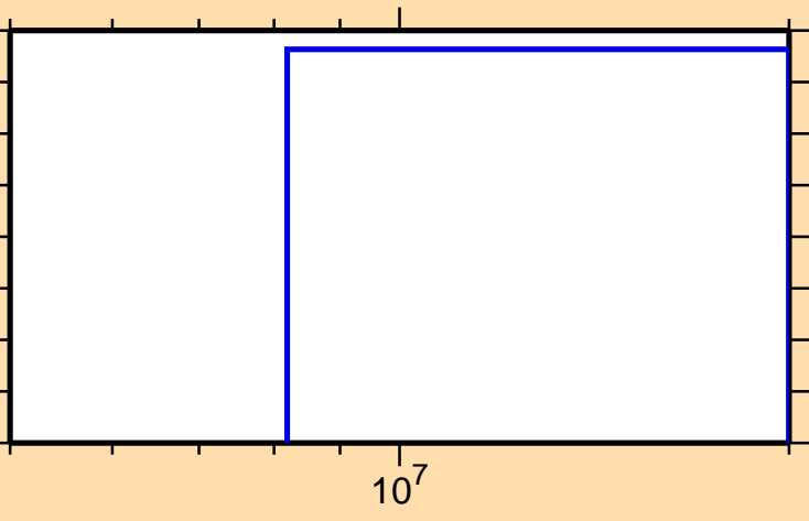
\sigma vs. E for ^{151}\text{Dy}(n,3n)
