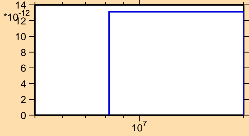
\sigma vs. E for ^{151}\text{Dy} (mt 34)
