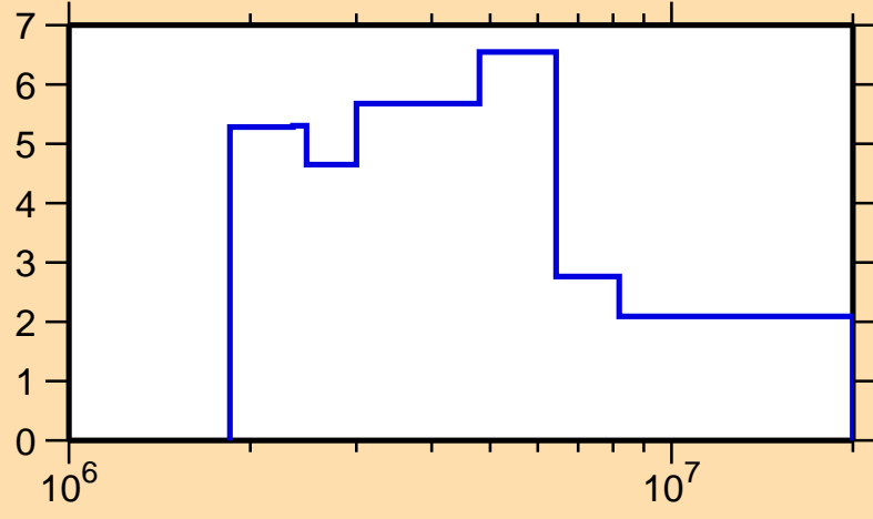
\Delta\sigma/\sigma vs. E for ^{151}\text{Dy}(n,\text{tot.})
