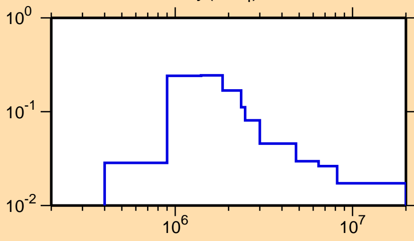
\sigma vs. E for ^{151}\text{Dy}(n,n_4)
