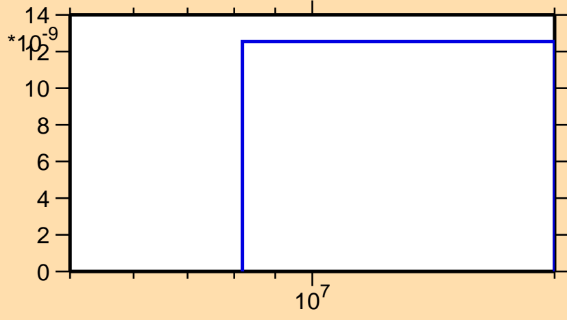
\sigma vs. E for ^{151}\text{Dy} (mt 45)
