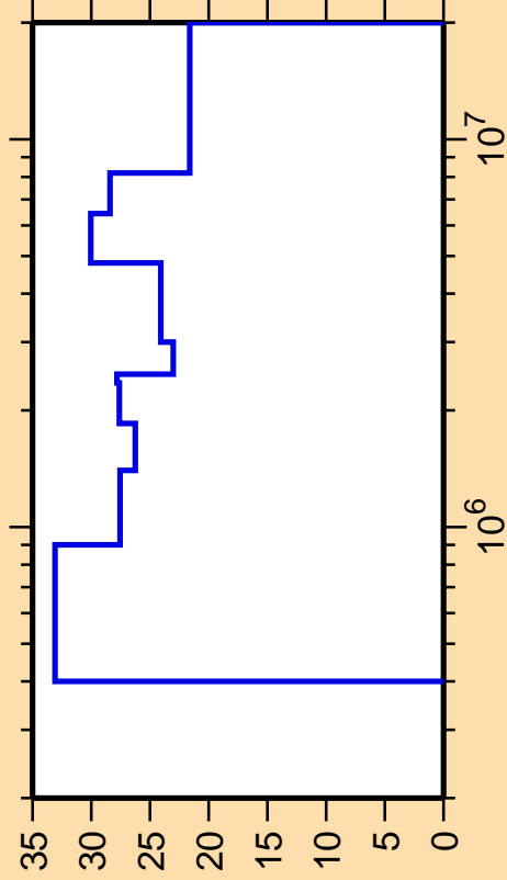
\Delta\sigma/\sigma vs. E for ^{151}\text{Dy}(n,n_4)
