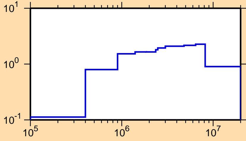
\sigma vs. E for ^{151}\text{Dy}(n,\text{inel.})
