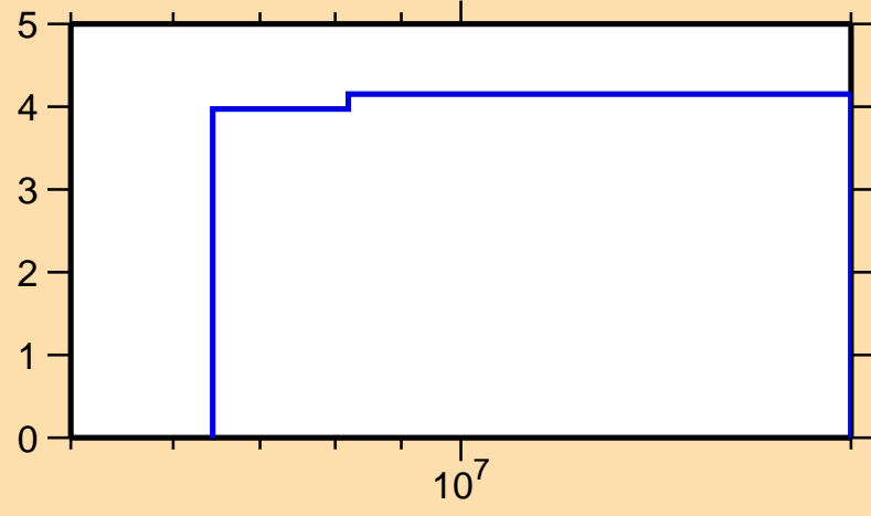
\Delta\sigma/\sigma vs. E for ^{151}\text{Dy}(n,\text{el.})
