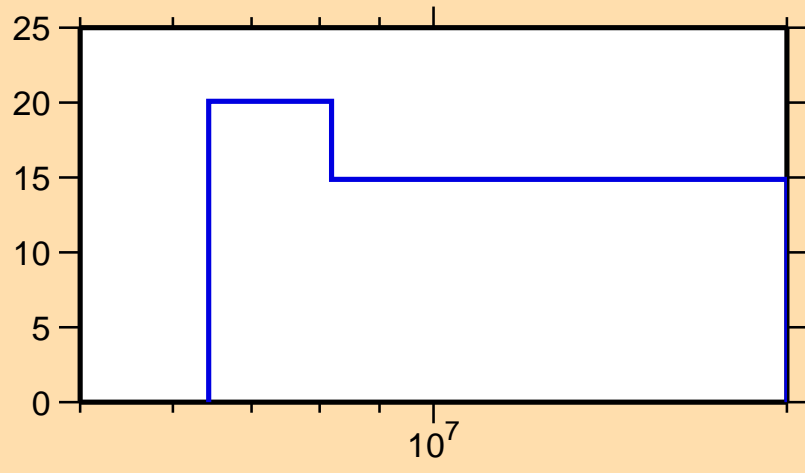
\Delta\sigma/\sigma vs. E for ^{151}\text{Dy}(n,2n)
