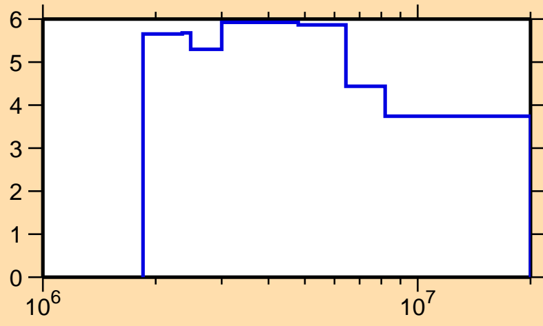
\Delta\sigma/\sigma vs. E for ^{151}\text{Dy}(n,\text{nonel.})
