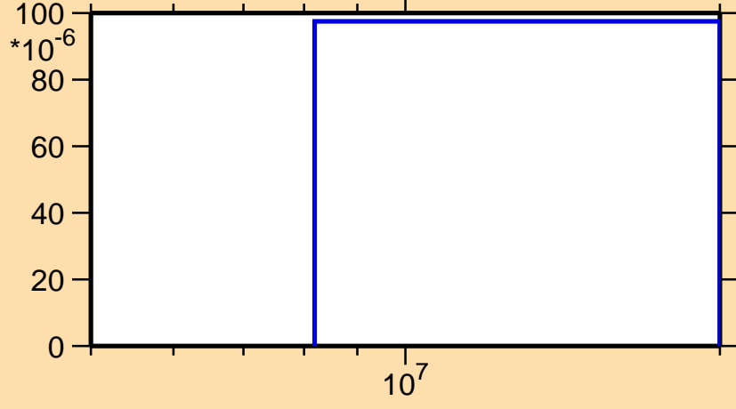
\sigma vs. E for ^{151}\text{Dy}(n,2n\alpha)
