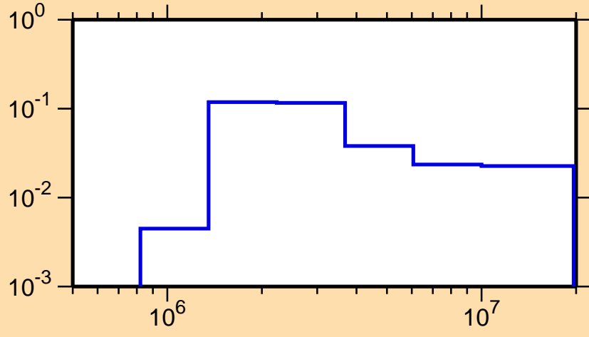
\sigma vs. E for ^{152}\text{Dy}(n,n_2)
