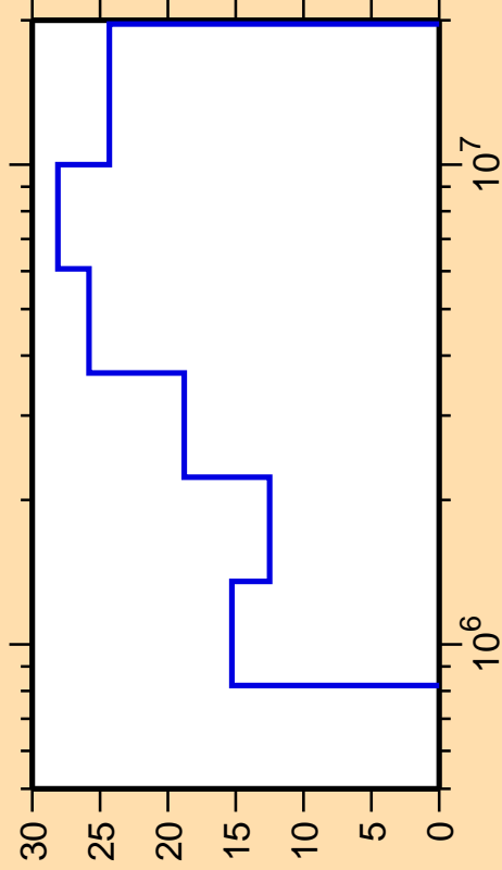
\Delta\sigma/\sigma vs. E for ^{152}\text{Dy}(n,n_4)
