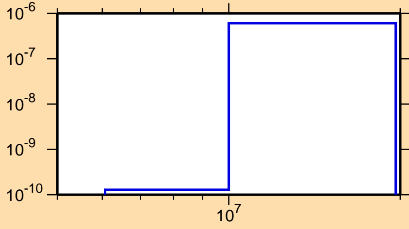
\sigma vs. E for ^{152}\text{Dy}(n,p\alpha)
