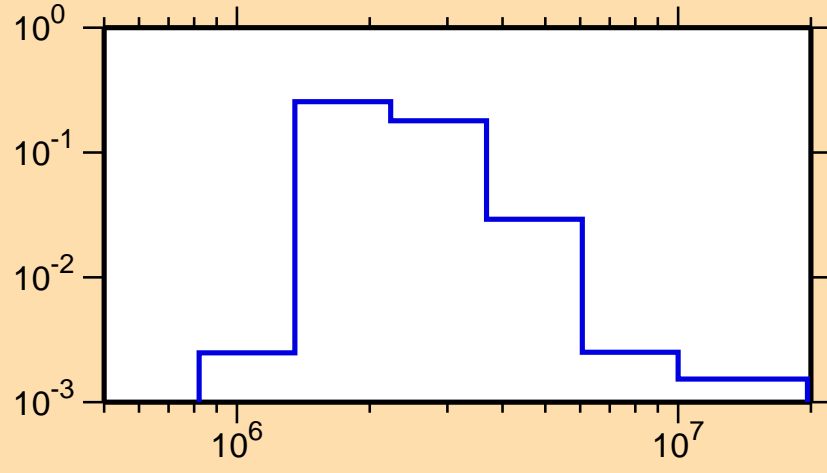
\sigma vs. E for ^{152}\text{Dy}(n,n_4)
