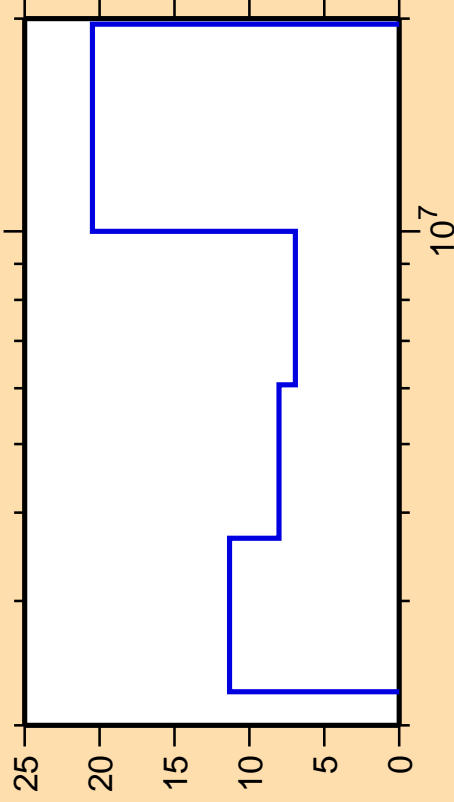
\Delta\sigma/\sigma vs. E for ^{152}\text{Dy}(n,\text{ncont.})
