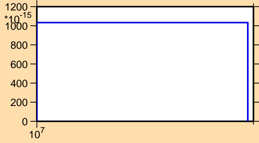
\sigma vs. E for ^{152}\text{Dy}(n,pt)
