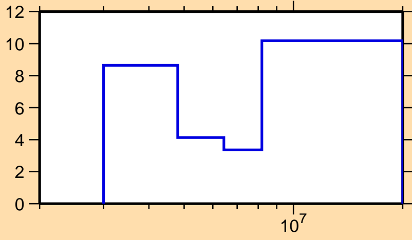
\Delta\sigma/\sigma vs. E for ^{152}\text{Dy}(n,inel.)
