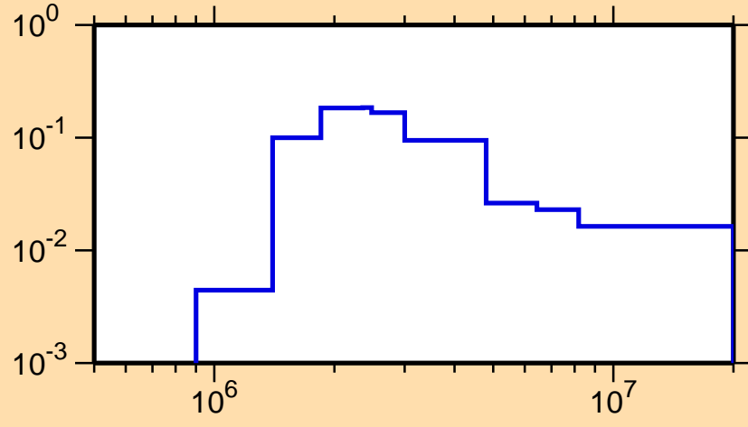
\sigma vs. E for ^{152}\text{Dy}(n,n_3)
