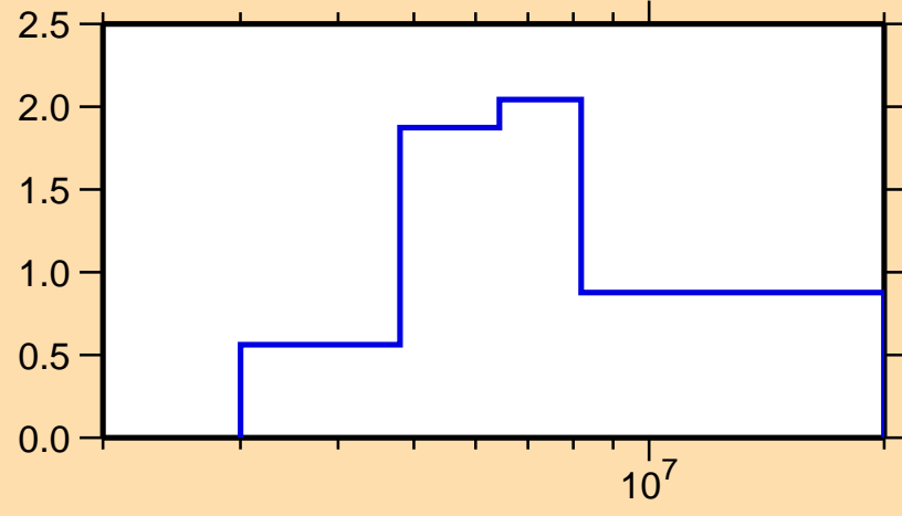
\sigma vs. E for ^{152}\text{Dy}(n,n\text{cont.})
