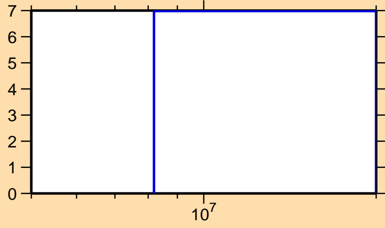
\Delta\sigma/\sigma vs. E for ^{152}\text{Dy}(n,2n)
