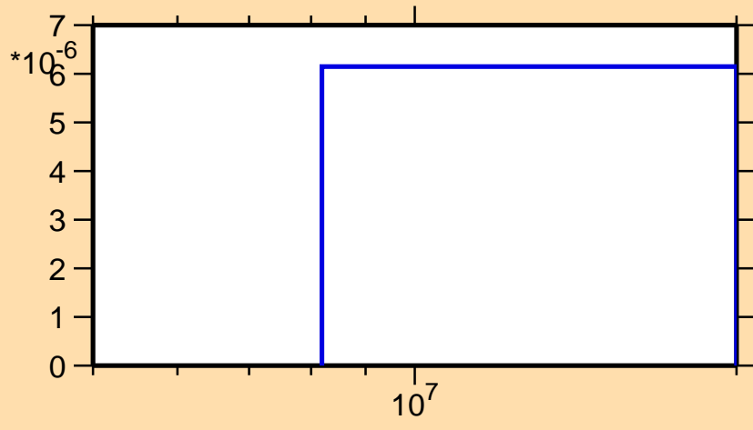
\sigma vs. E for ^{152}\text{Dy}(n,2n\alpha)
