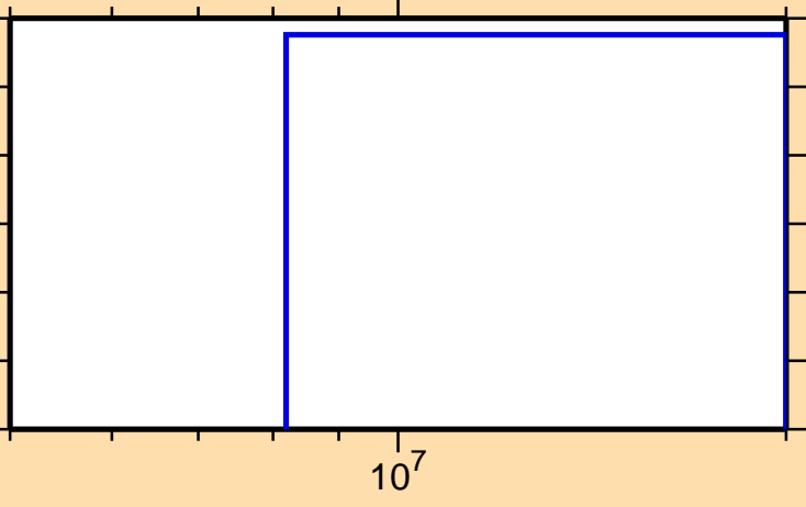
\sigma vs. E for ^{152}\text{Dy}(\text{mt117})
