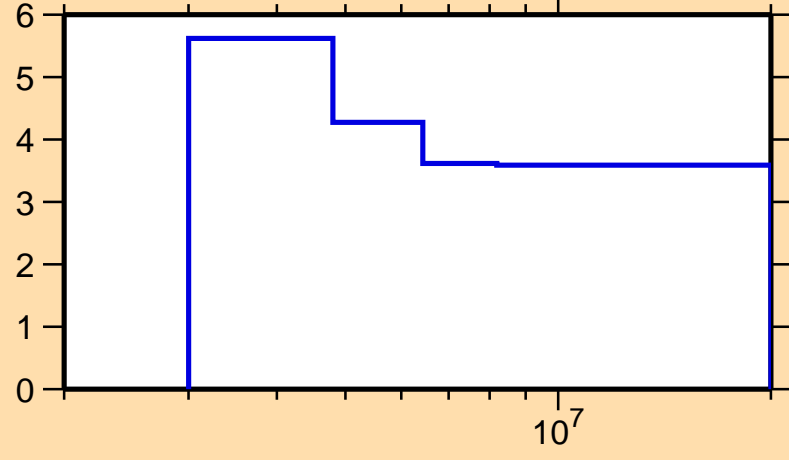
\Delta\sigma/\sigma vs. E for ^{152}\text{Dy}(n,\text{nonel.})
