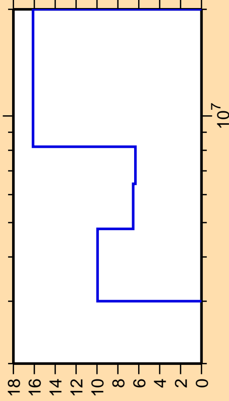
\Delta\sigma/\sigma vs. E for ^{152}\text{Dy}(n,ncont.)
