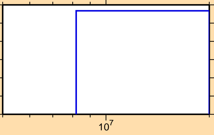
\sigma vs. E for ^{152}\text{Dy}(n,\text{He}3)
