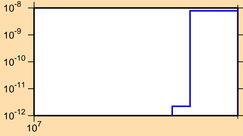
\sigma vs. E for ^{153}\text{Dy}(n,nt)
