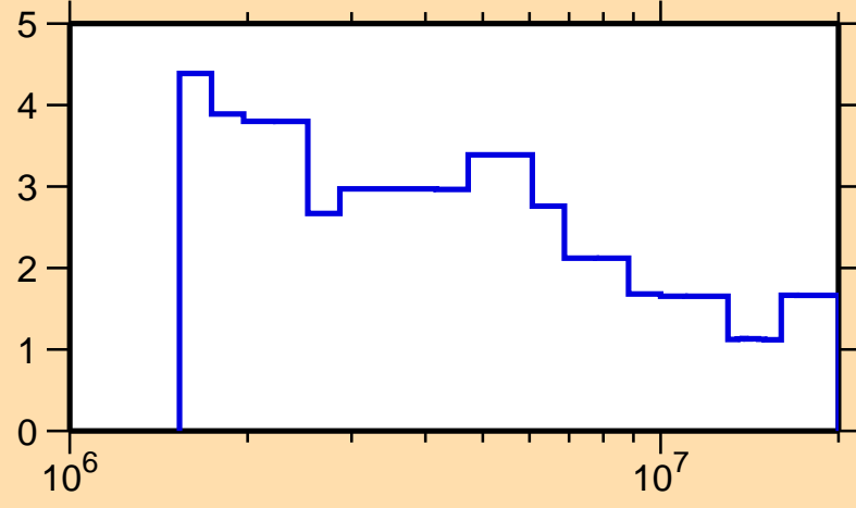
\Delta\sigma/\sigma vs. E for ^{153}\text{Dy}(n, tot.)
