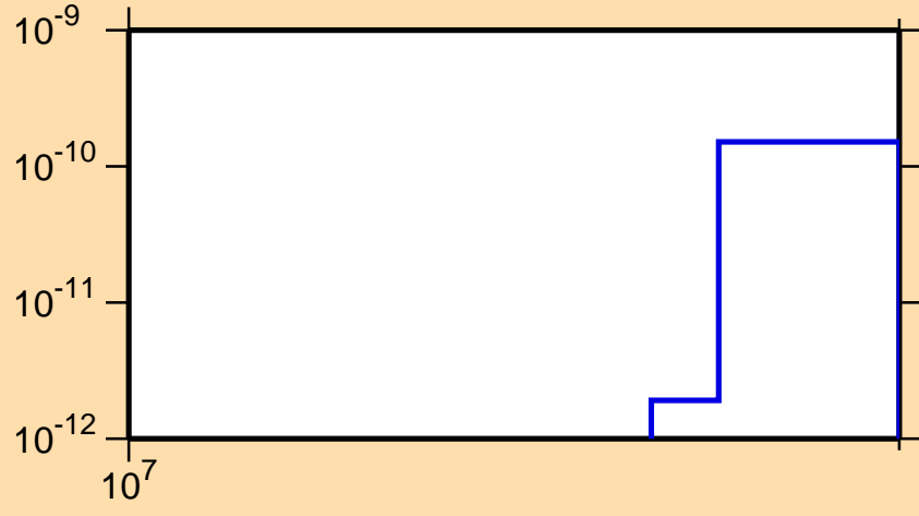
\sigma vs. E for ^{153}\text{Dy} (mt 34)
