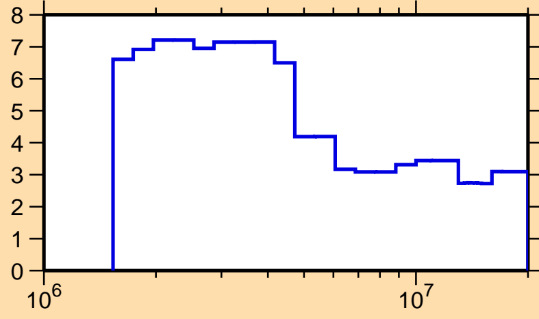
\Delta\sigma/\sigma vs. E for ^{153}\text{Dy}(n,\text{el.})
