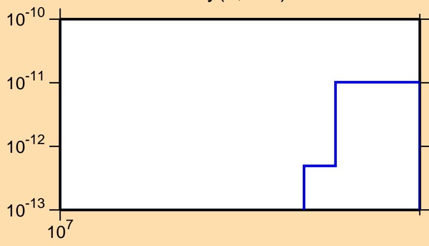
\sigma vs. E for ^{153}\text{Dy}(n,3n\alpha)
