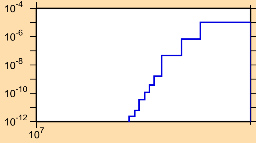
\sigma vs. E for ^{153}\text{Dy}(n,nd)
