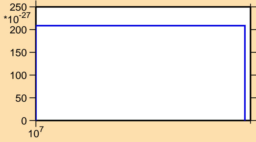
\sigma vs. E for ^{153}\text{Dy} (mt 11)
