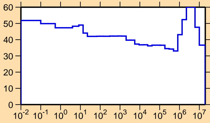
\Delta\sigma/\sigma vs. E for ^{153}\text{Dy}(n,p)
