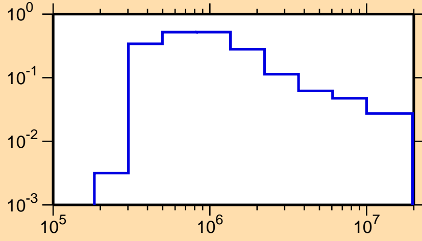
\sigma vs. E for ^{153}\text{Dy}(n,n_3)
