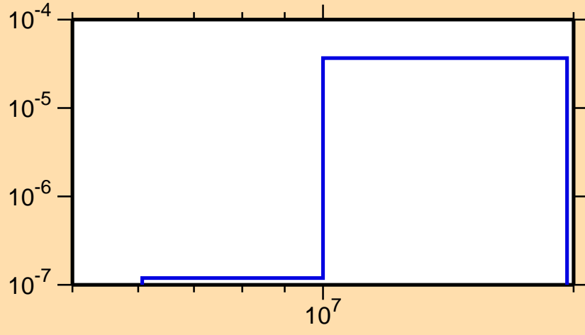
\sigma vs. E for ^{153}\text{Dy}(n,2n\alpha)
