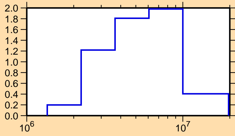
\sigma vs. E for ^{153}\text{Dy}(n,n\text{cont.})
