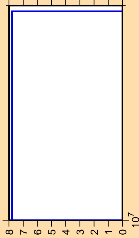
\Delta\sigma/\sigma vs. E for ^{153}\text{Dy} (mt 34)
