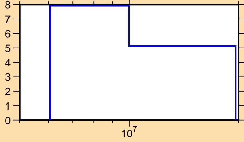
\Delta\sigma/\sigma vs. E for ^{153}\text{Dy}(n,2n)
