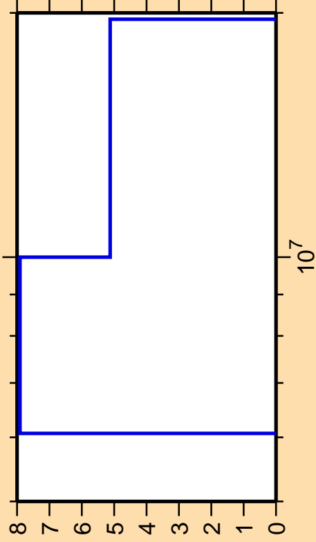
\Delta\sigma/\sigma vs. E for ^{153}\text{Dy}(n,2n)
