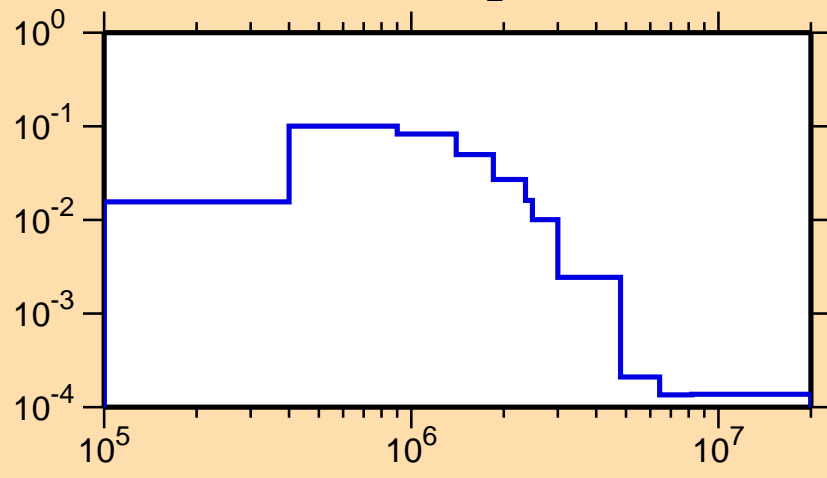
\sigma vs. E for ^{153}\text{Dy}(n,n_2)
