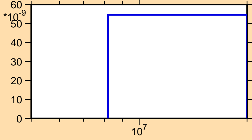
\sigma vs. E for ^{153}\text{Dy}(n,\text{He}3)
