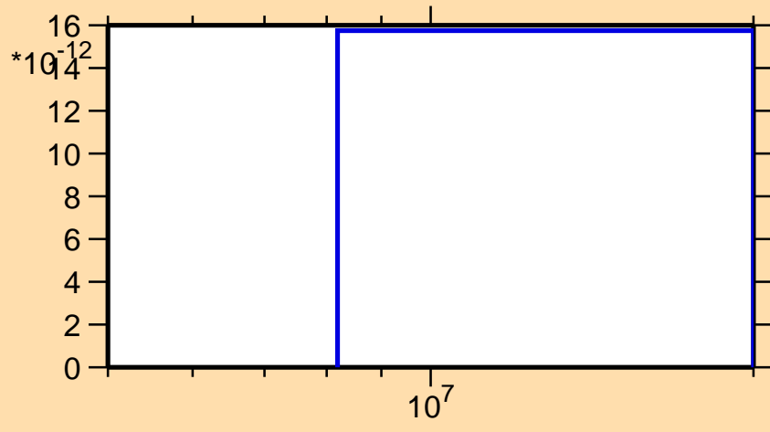
\sigma vs. E for ^{153}\text{Dy}(n,\text{pd})
