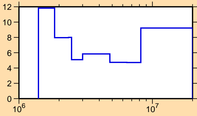
\Delta\sigma/\sigma vs. E for ^{153}\text{Dy}(n,inel.)
