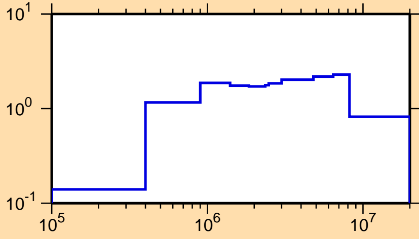
\sigma vs. E for ^{153}\text{Dy}(n,\text{inel.})
