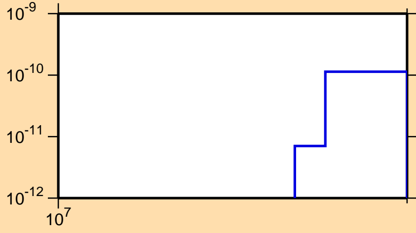
\sigma vs. E for ^{154}\text{Dy}(\text{mt117})
