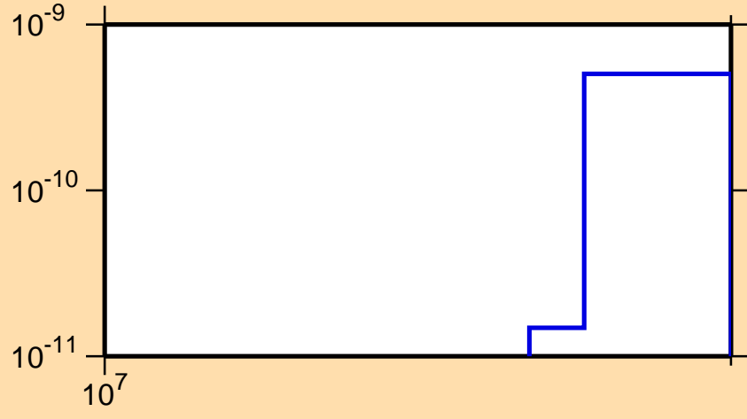
\sigma vs. E for ^{154}\text{Dy}(n,\text{pd})
