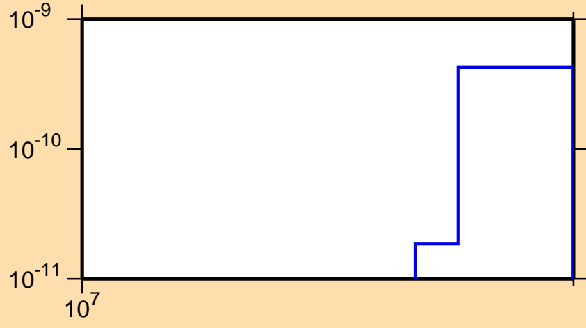
\sigma vs. E for ^{154}\text{Dy} (mt 45)
