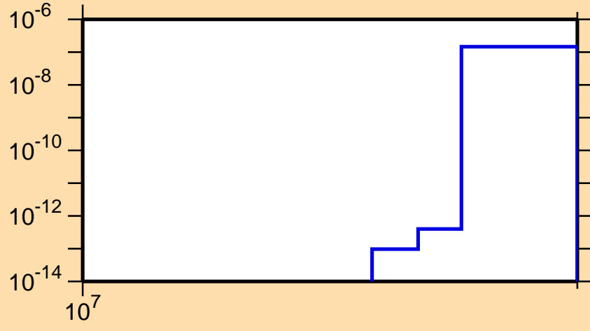
\sigma vs. E for ^{154}\text{Dy}(n,2np)
