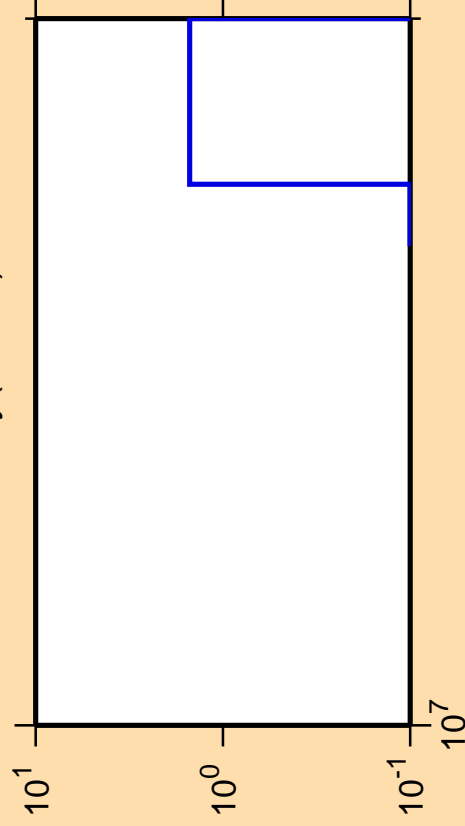
\Delta\sigma/\sigma vs. E for ^{154}\text{Dy} (mt 34)
