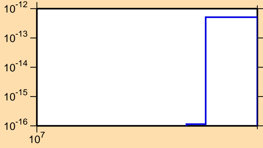
\sigma vs. E for ^{154}\text{Dy}(n,pt)
