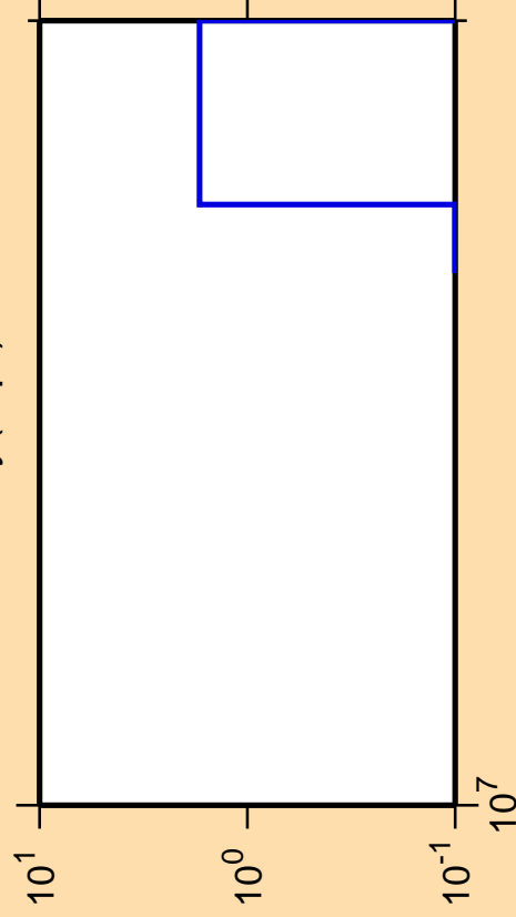
\Delta\sigma/\sigma vs. E for ^{154}\text{Dy}(n,pt)
