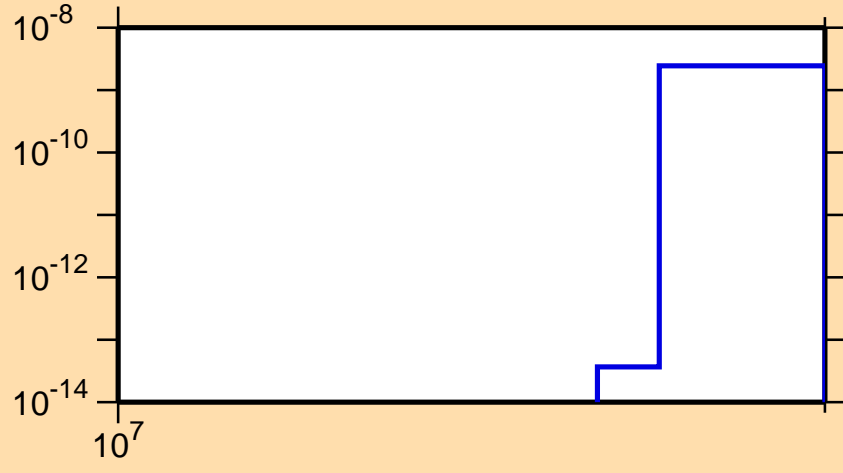
\sigma vs. E for ^{154}\text{Dy}(n,nt)
