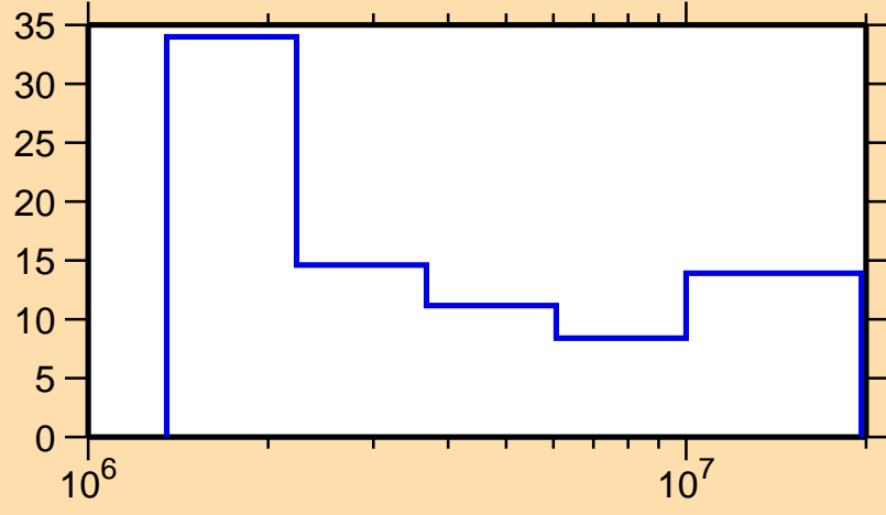
\Delta\sigma/\sigma vs. E for ^{154}\text{Dy}(n,n\text{cont.})
