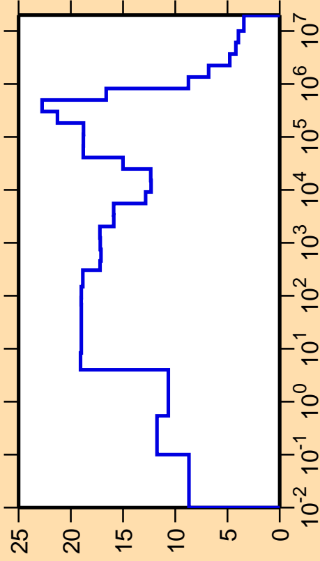
\Delta\sigma/\sigma vs. E for ^{154}\text{Dy}(n,\text{nonel.})
