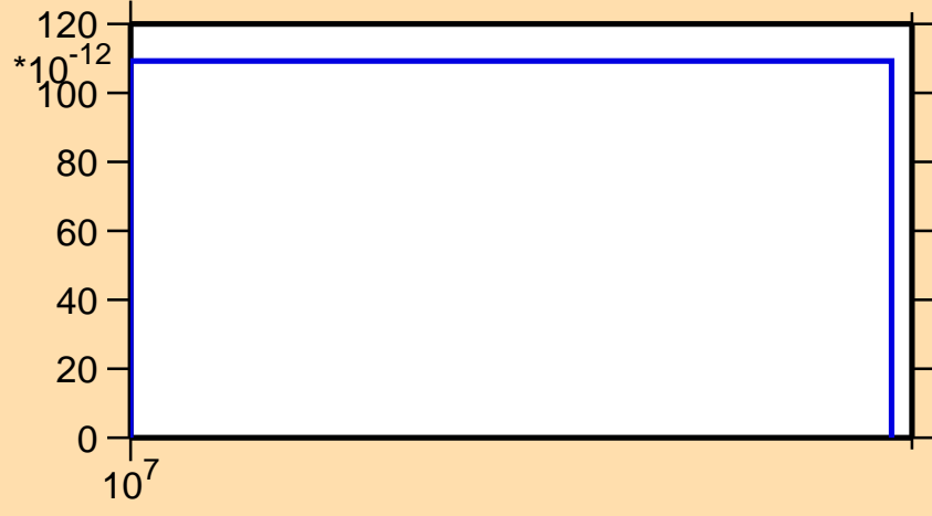
\sigma vs. E for ^{154}\text{Dy}(n,3n\alpha)
