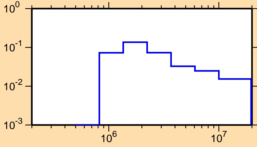
\sigma vs. E for ^{154}\text{Dy}(n,n_3)
