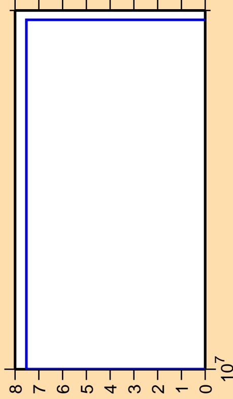
\Delta\sigma/\sigma vs. E for ^{154}\text{Dy}(n,pd)
