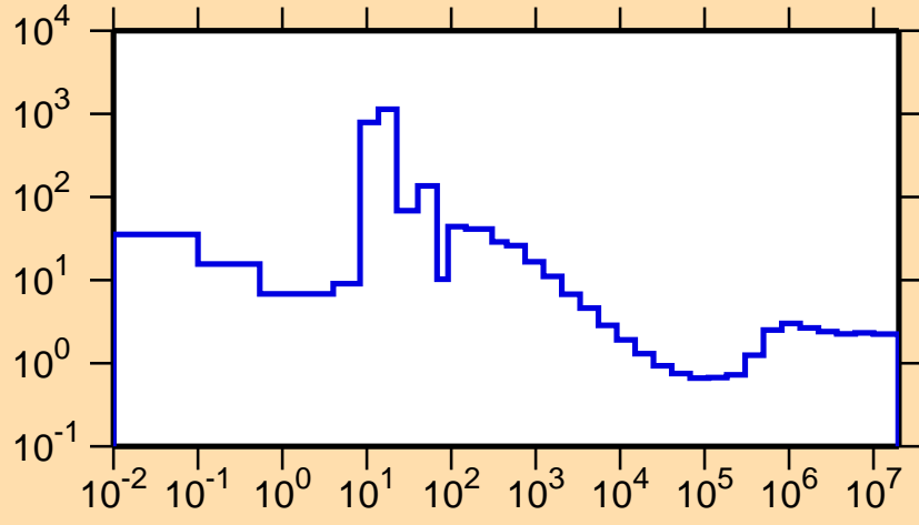
\sigma vs. E for ^{154}\text{Dy}(n,\text{nonel.})
