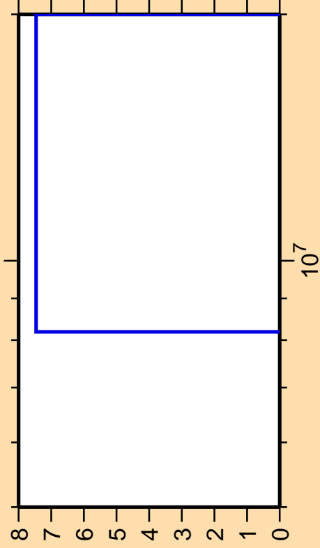
\Delta\sigma/\sigma vs. E for ^{154}\text{Dy}(n,2n)
