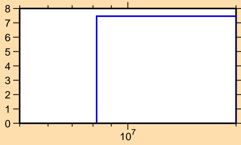
\Delta\sigma/\sigma vs. E for ^{154}\text{Dy}(n,2n)
