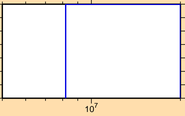
\sigma vs. E for ^{154}\text{Dy}(n,nd)
