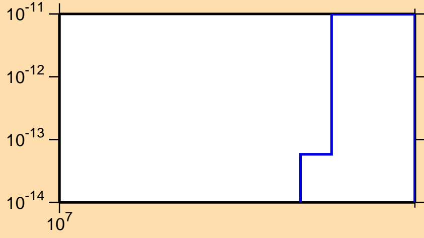
\sigma vs. E for ^{156}\text{Dy}(n,\text{pd})
