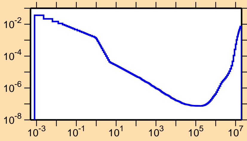
\sigma vs. E for ^{156}\text{Dy}(n,\alpha)
