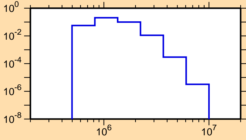
\sigma vs. E for ^{156}\text{Dy}(n,n_3)
