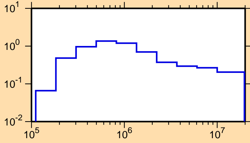
\sigma vs. E for ^{156}\text{Dy}(n,n_1)
