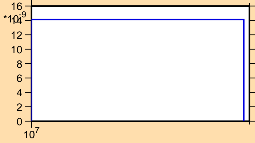
\sigma vs. E for ^{156}\text{Dy}(n,2n\alpha)
