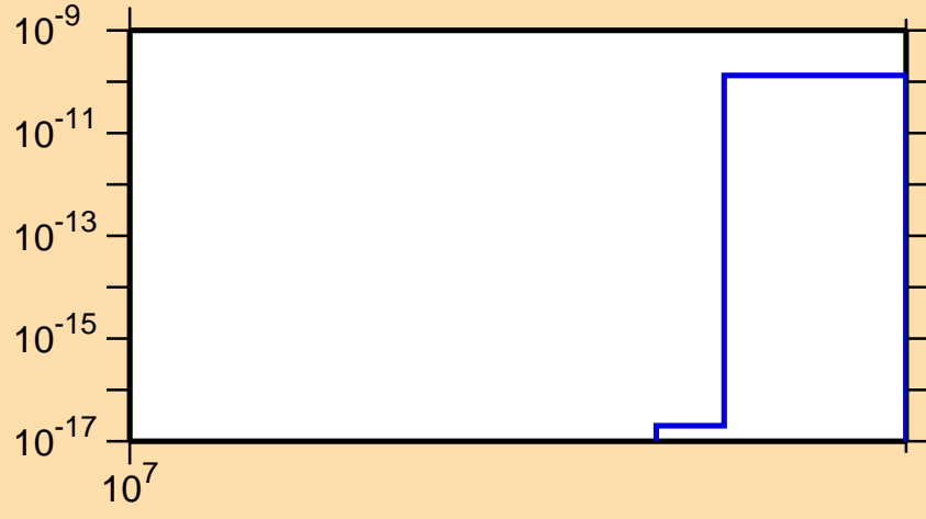
\sigma vs. E for ^{157}\text{Dy}(n,nt)
