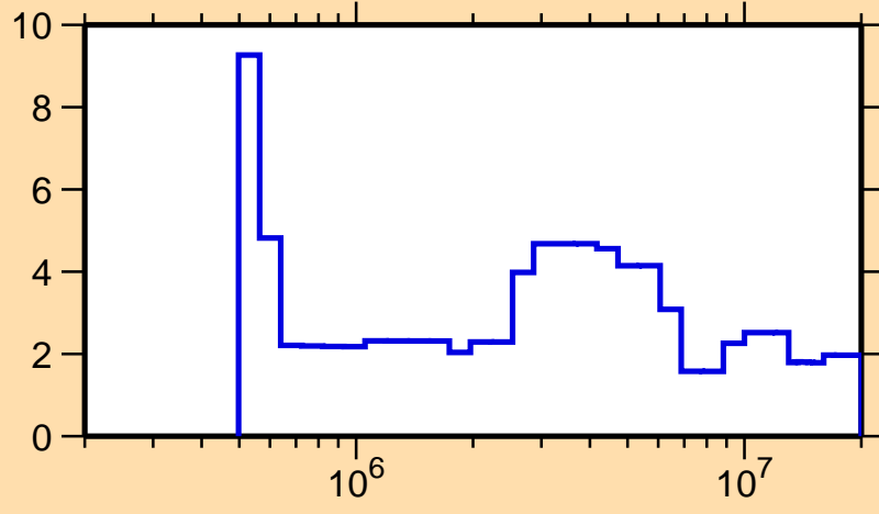
\Delta\sigma/\sigma vs. E for ^{157}\text{Dy}(n,el.)
