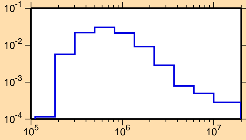
\sigma vs. E for ^{157}\text{Dy}(n,n_3)
