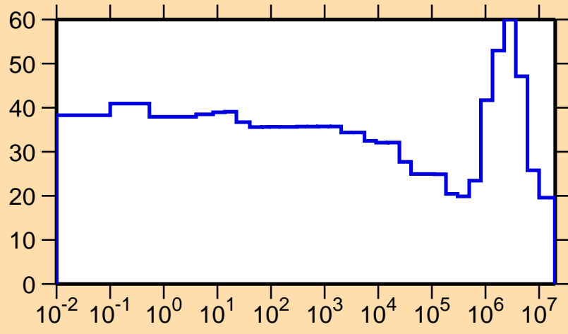
\Delta\sigma/\sigma vs. E for ^{157}\text{Dy}(n,p)
