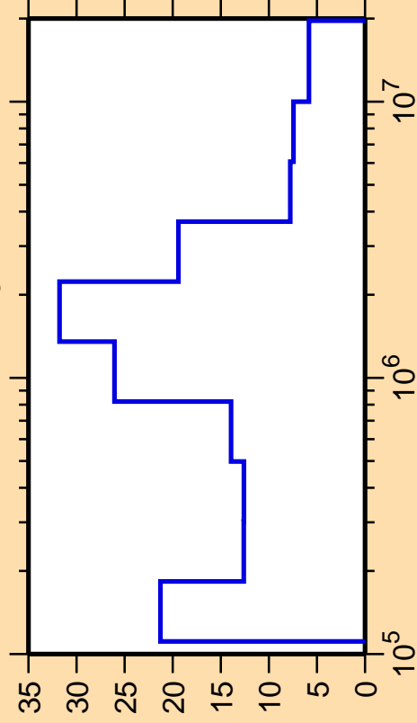
\Delta\sigma/\sigma vs. E for ^{157}\text{Dy}(n,n_3)
