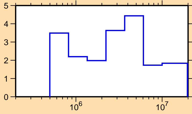
\Delta\sigma/\sigma vs. E for ^{157}\text{Dy}(n,el.)
