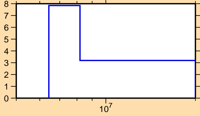
\Delta\sigma/\sigma vs. E for ^{157}\text{Dy}(n,2n)
