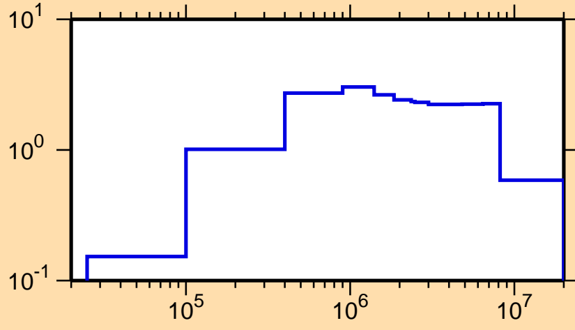
\sigma vs. E for ^{157}\text{Dy}(n,\text{inel.})
