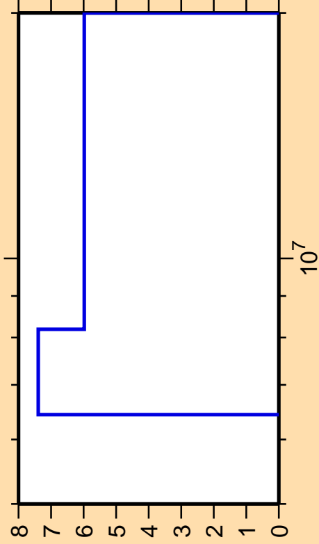
\Delta\sigma/\sigma vs. E for ^{157}\text{Dy}(n,n_1)
