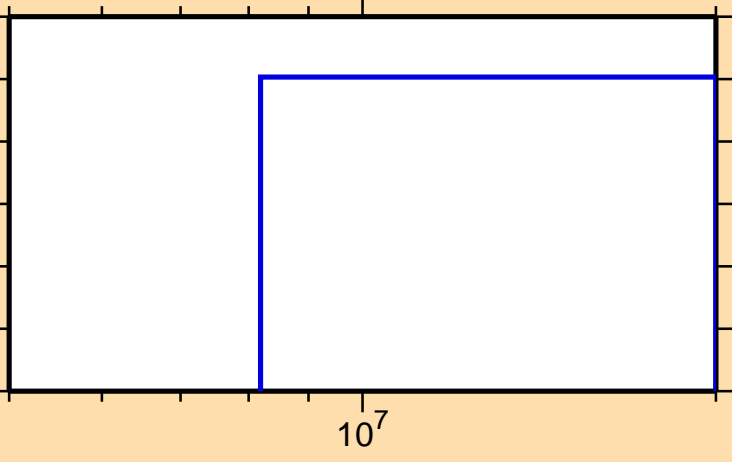
\sigma vs. E for ^{157}\text{Dy}(n,t)
