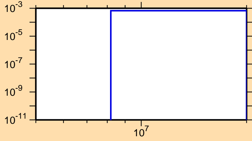
\sigma vs. E for ^{157}\text{Dy}(n,np)
