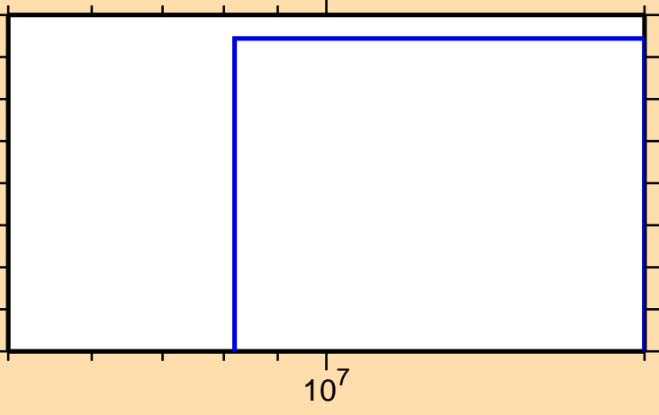
\sigma vs. E for ^{157}\text{Dy}(n,3n)
