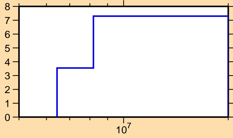
\Delta\sigma/\sigma vs. E for ^{157}\text{Dy}(n,\text{inel.})
