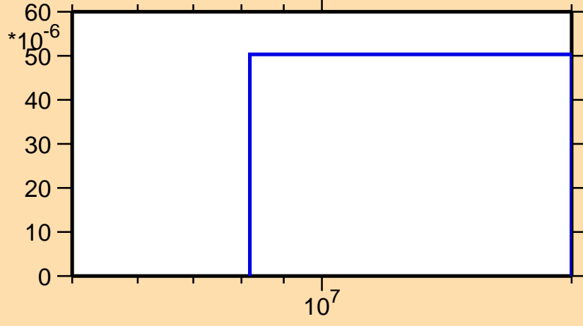
\sigma vs. E for ^{157}\text{Dy}(n,t)
