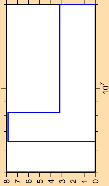
\Delta\sigma/\sigma vs. E for ^{157}\text{Dy}(n,2n)
