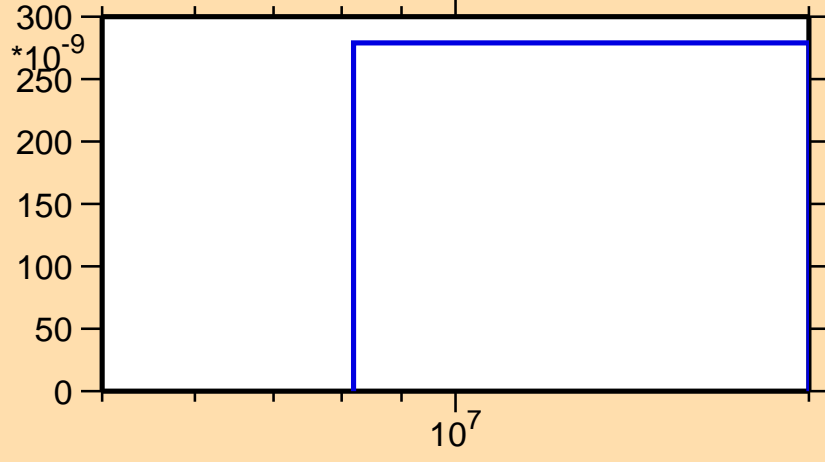
\sigma vs. E for ^{157}\text{Dy}(n,2n\alpha)
