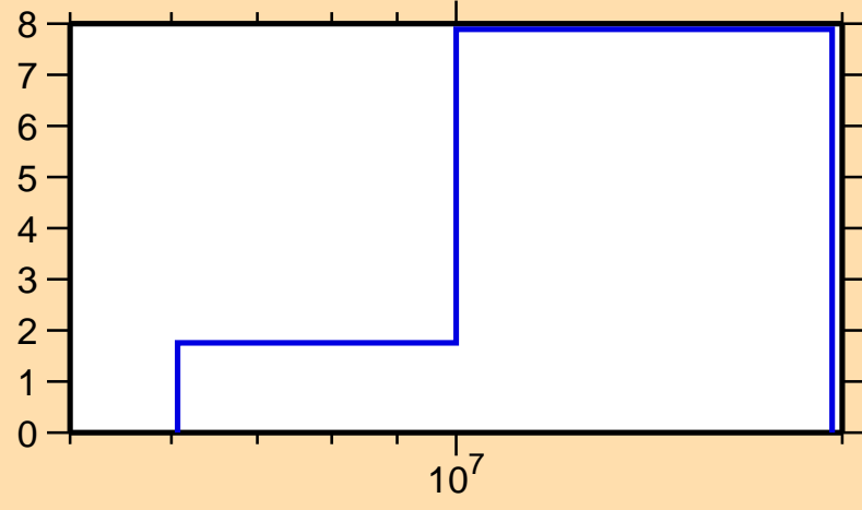
\Delta\sigma/\sigma vs. E for ^{158}\text{Dy}(n,\text{inel.})
