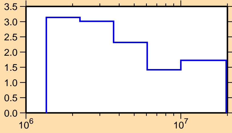
\Delta\sigma/\sigma vs. E for ^{158}\text{Dy}(n, tot.)
