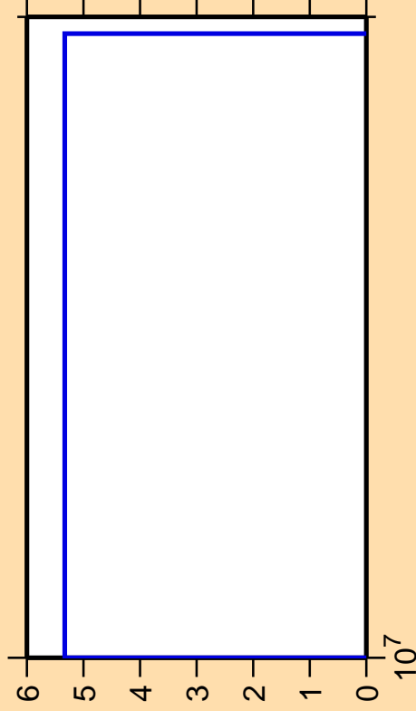
\Delta\sigma/\sigma vs. E for ^{158}\text{Dy}(n,nt)
