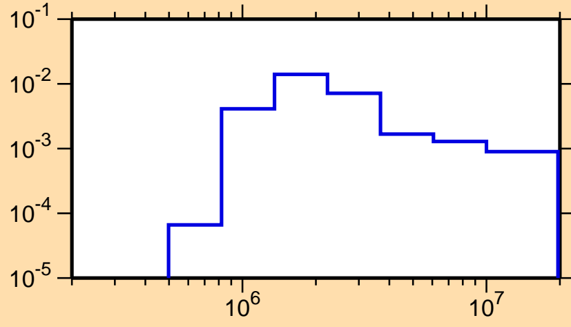
\sigma vs. E for ^{158}\text{Dy}(n,n_3)
