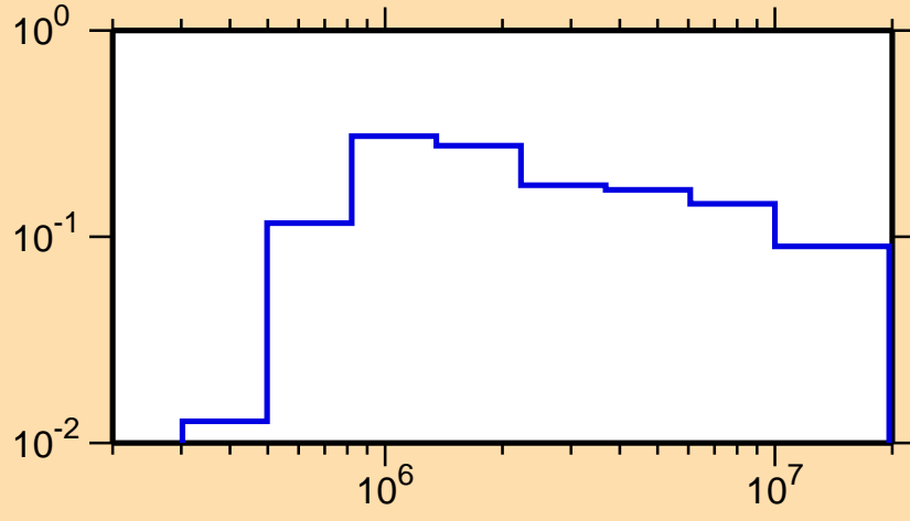
\sigma vs. E for ^{158}\text{Dy}(n,n_2)
