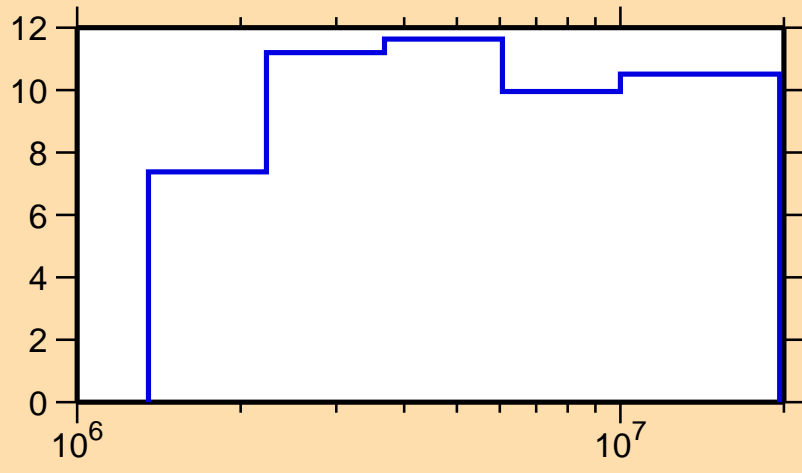
\Delta\sigma/\sigma vs. E for ^{158}\text{Dy}(n,n_1)
