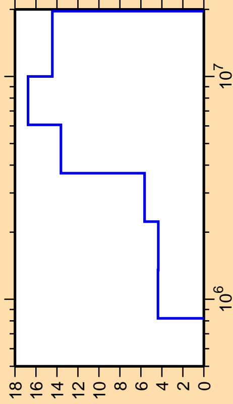
\Delta\sigma/\sigma vs. E for ^{158}\text{Dy}(n,n_4)
