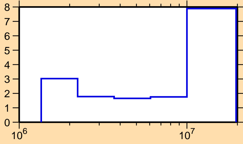
\Delta\sigma/\sigma vs. E for ^{158}\text{Dy}(n,inel.)
