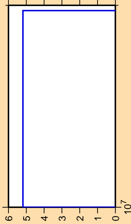
\Delta\sigma/\sigma vs. E for ^{158}\text{Dy}(n,2np)
