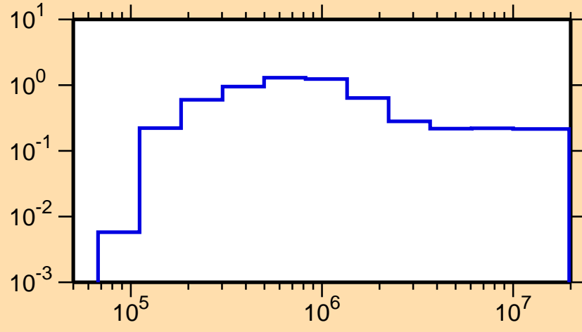
\sigma vs. E for ^{158}\text{Dy}(n,n_1)
