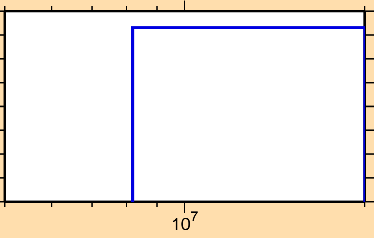
\sigma vs. E for ^{158}\text{Dy}(n,3n)
