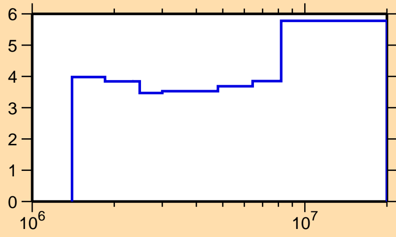
\Delta\sigma/\sigma vs. E for ^{158}\text{Dy}(n,n\text{cont.})
