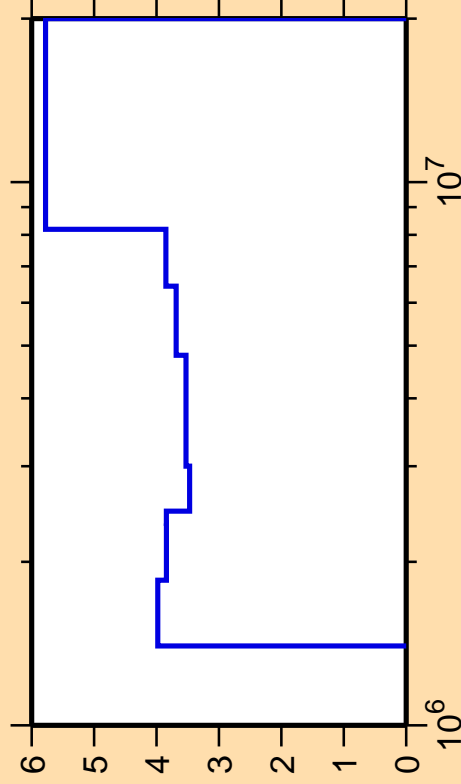
\Delta\sigma/\sigma vs. E for ^{158}\text{Dy}(n,n\text{cont.})
