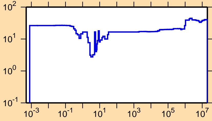
\Delta\sigma/\sigma vs. E for ^{159}\text{Dy}(n,\gamma)
