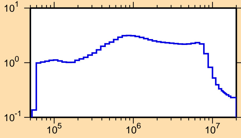
\sigma vs. E for ^{159}\text{Dy}(n,\text{inel.})
