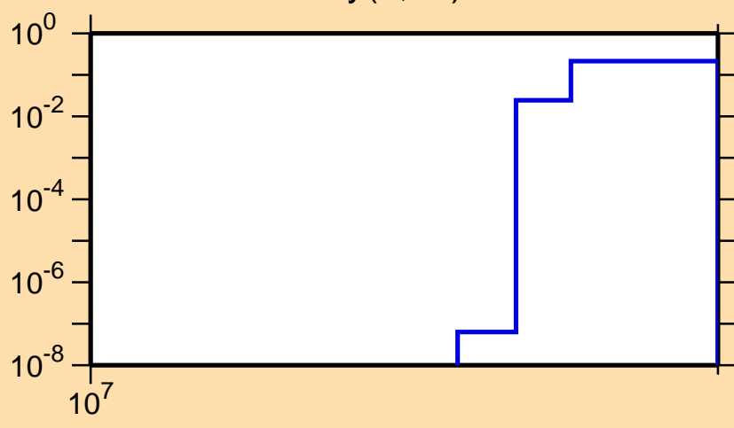
\sigma vs. E for ^{159}\text{Dy}(n,3n)
