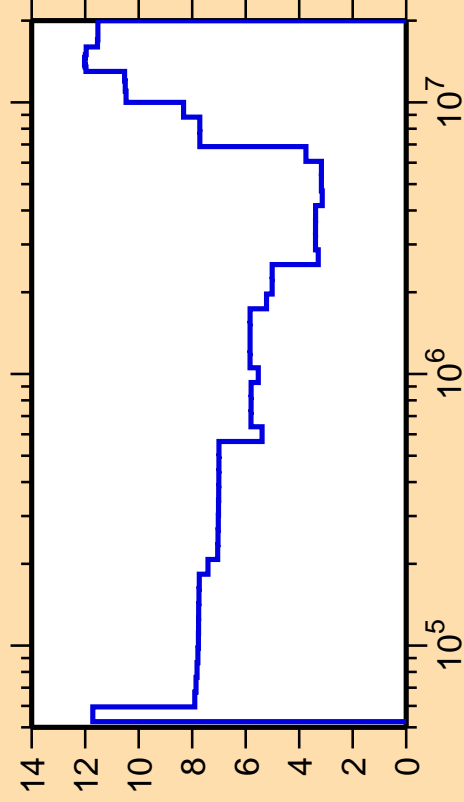
\Delta\sigma/\sigma vs. E for ^{159}\text{Dy}(n,\text{inel.})
