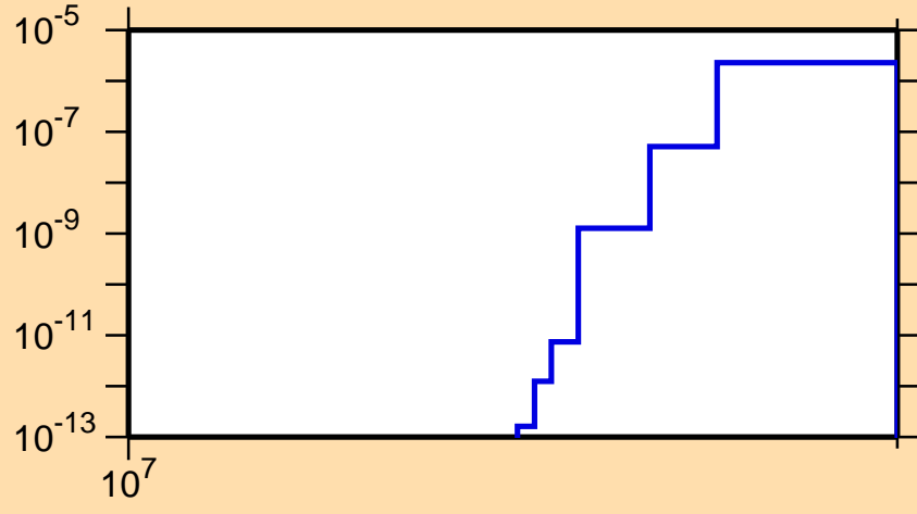
\sigma vs. E for ^{159}\text{Dy}(n,nd)
