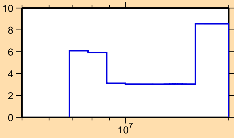
\Delta\sigma/\sigma vs. E for ^{159}\text{Dy}(n,2n)
