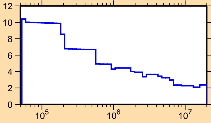
\Delta\sigma/\sigma vs. E for ^{159}\text{Dy}(n,\text{nonel.})
