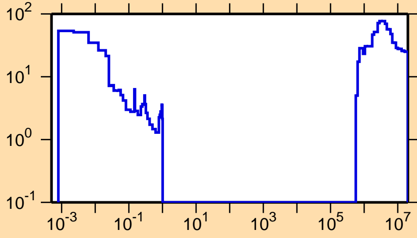
\Delta\sigma/\sigma vs. E for ^{159}\text{Dy}(n,p)
