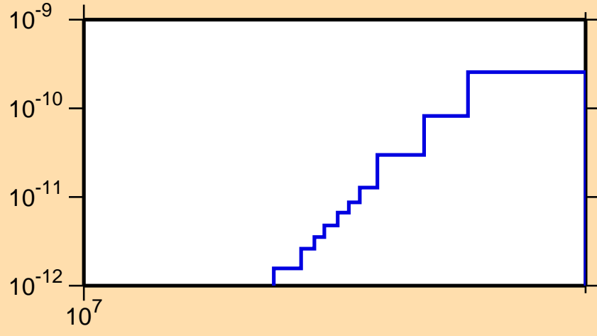
\sigma vs. E for ^{159}\text{Dy}(n,p\alpha)
