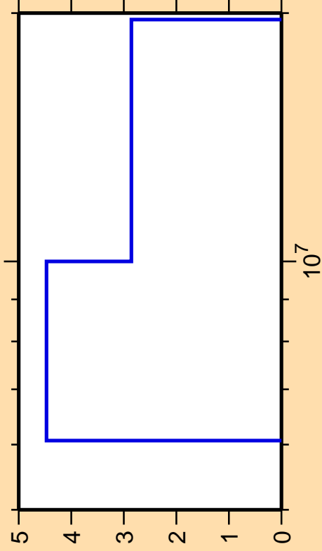
\Delta\sigma/\sigma vs. E for ^{159}\text{Dy}(n,2n)
