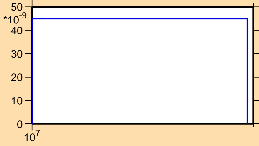
\sigma vs. E for ^{159}\text{Dy}(n,2n\alpha)
