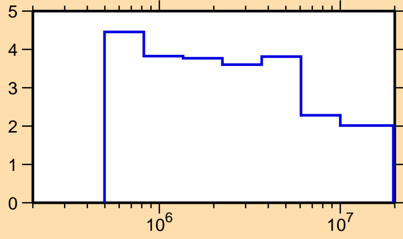
\Delta\sigma/\sigma vs. E for ^{159}\text{Dy}(n,\text{el.})
