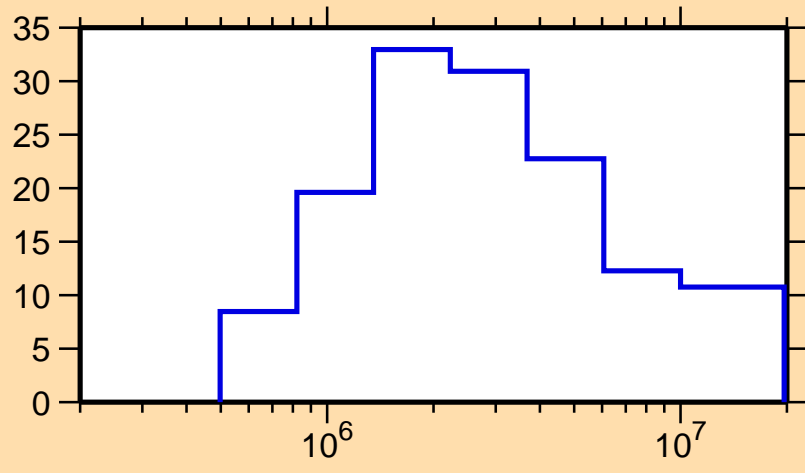
\Delta\sigma/\sigma vs. E for ^{159}\text{Dy}(n,n_1)
