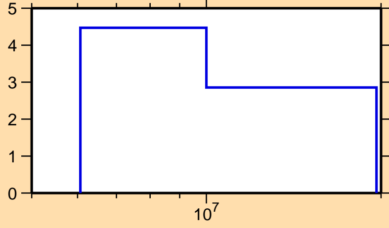
\Delta\sigma/\sigma vs. E for ^{159}\text{Dy}(n,2n)
