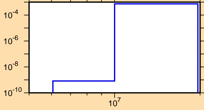
\sigma vs. E for ^{159}\text{Dy}(n,d)
