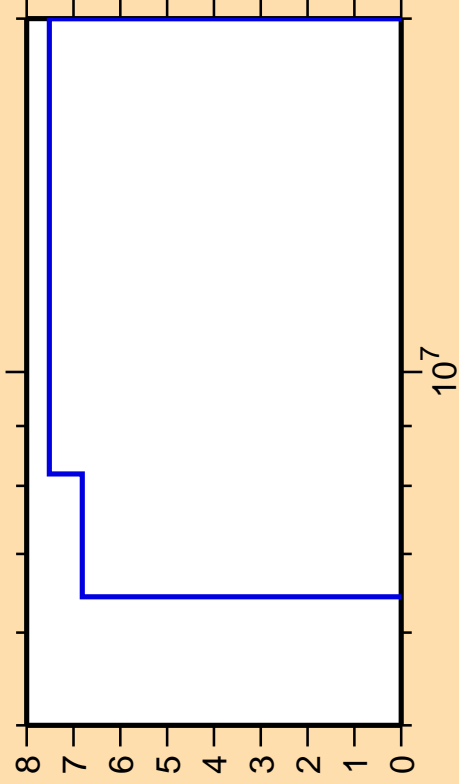
\Delta\sigma/\sigma vs. E for ^{159}\text{Dy}(n,n\text{cont.})
