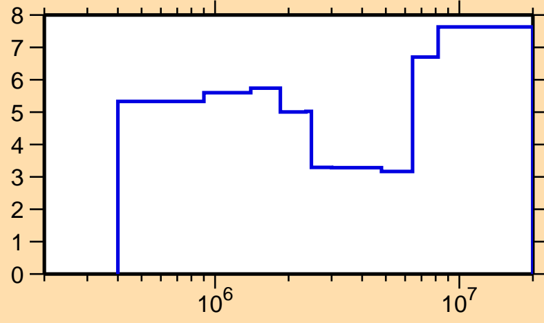
\Delta\sigma/\sigma vs. E for ^{159}\text{Dy}(n,\text{inel.})
