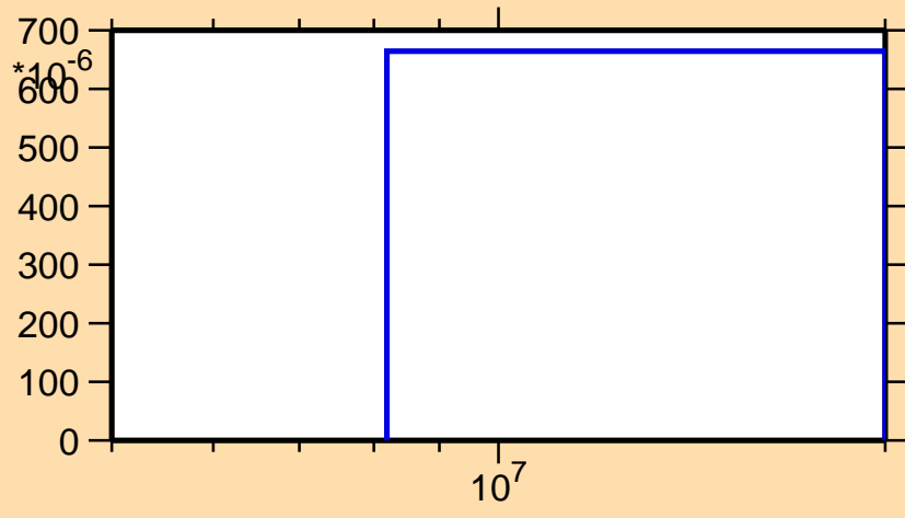
\sigma vs. E for ^{159}\text{Dy}(n,np)
