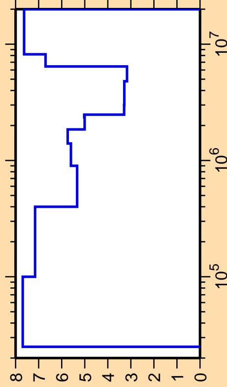
\Delta\sigma/\sigma vs. E for ^{159}\text{Dy}(n,\text{inel.})
