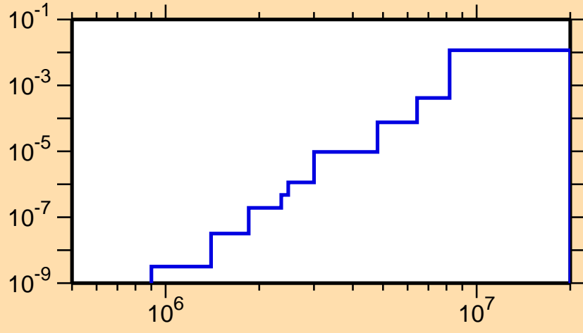
\sigma vs. E for ^{159}\text{Dy}(n,p)
