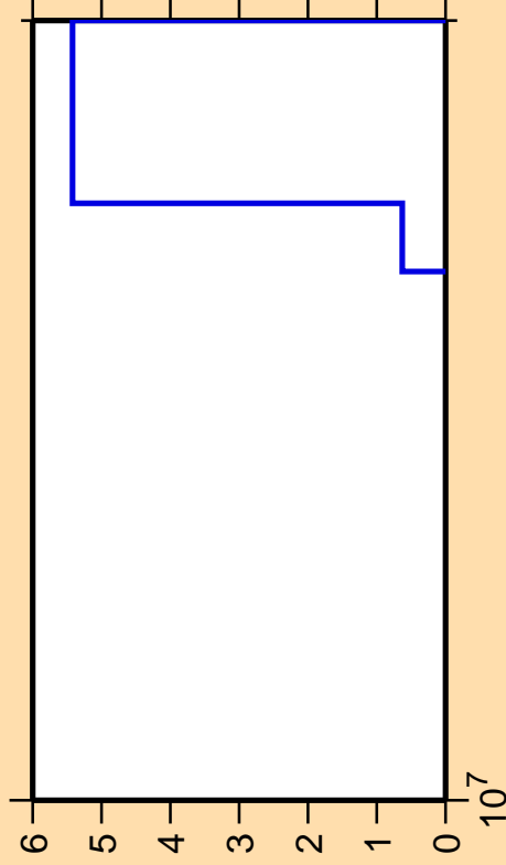
\Delta\sigma/\sigma vs. E for ^{160}\text{Dy}(n,p\alpha)
