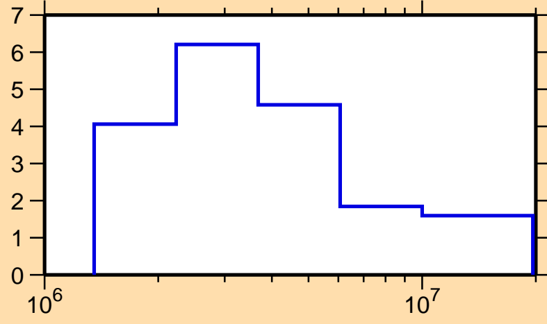
\Delta\sigma/\sigma vs. E for ^{160}\text{Dy}(n,el.)
