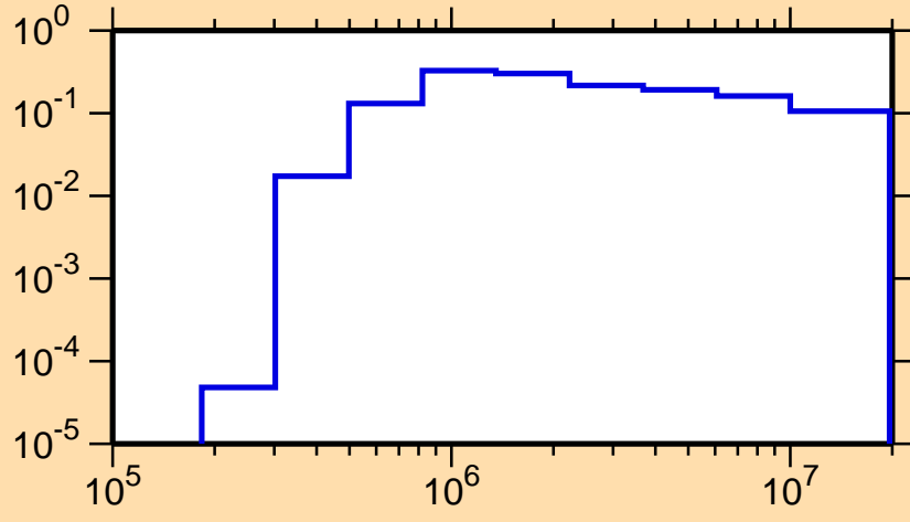
\sigma vs. E for ^{160}\text{Dy}(n,n_2)
