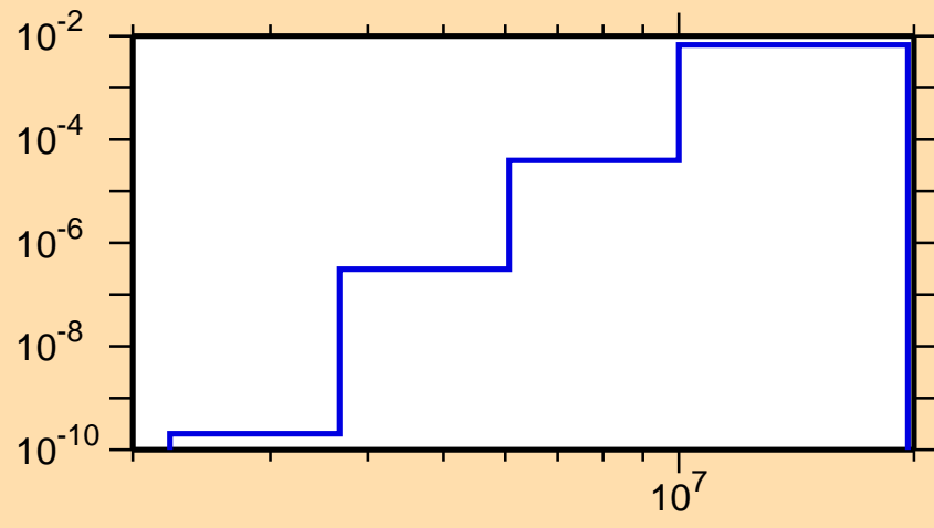
\sigma vs. E for ^{160}\text{Dy}(n,p)
