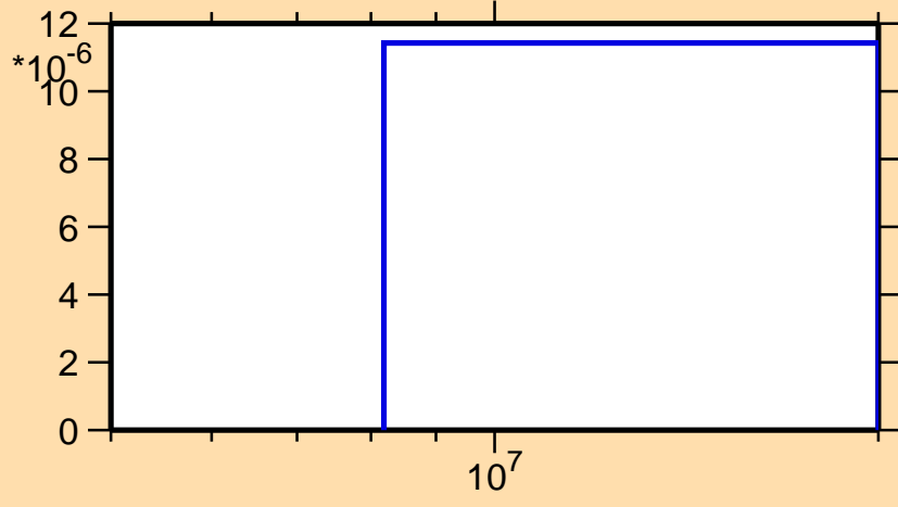
\sigma vs. E for ^{160}\text{Dy}(n,t)
