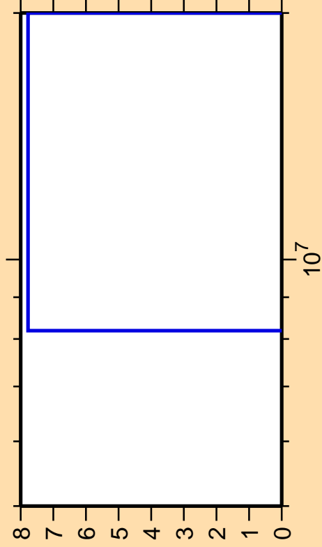
\Delta\sigma/\sigma vs. E for ^{160}\text{Dy}(n,n_1)
