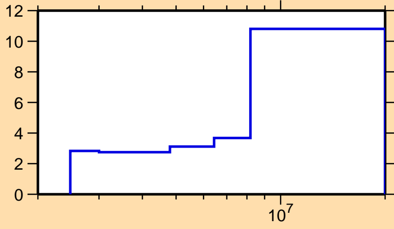
\Delta\sigma/\sigma vs. E for ^{160}\text{Dy}(n,n\text{cont.})
