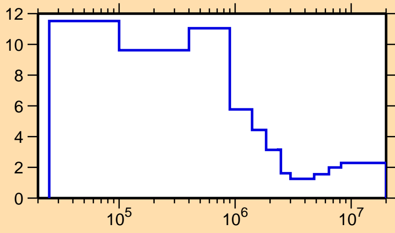
\Delta\sigma/\sigma vs. E for ^{160}\text{Dy}(n,\text{nonel.})
