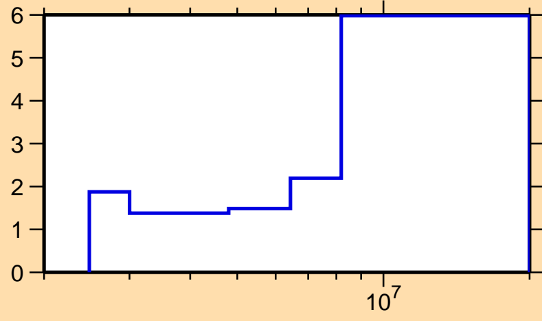
\Delta\sigma/\sigma vs. E for ^{160}\text{Dy}(n,\text{inel.})
