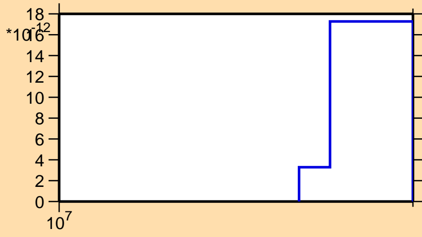
\sigma vs. E for ^{161}\text{Dy}(n,p\alpha)
