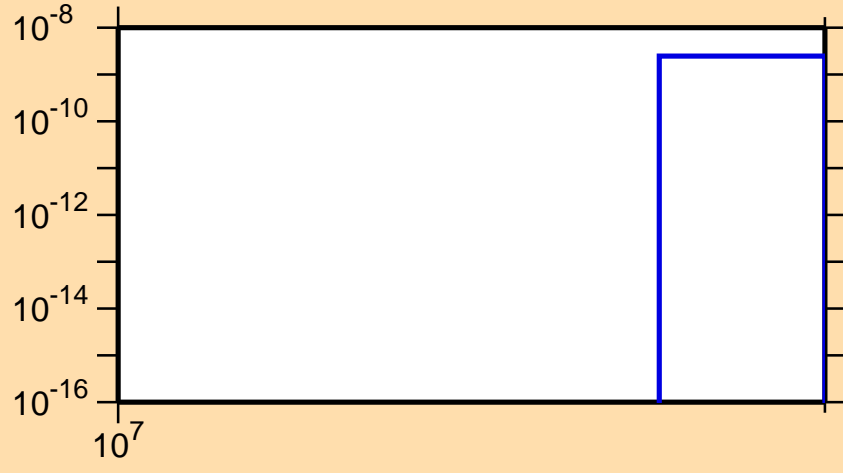
\sigma vs. E for ^{162}\text{Dy}(n,2np)
