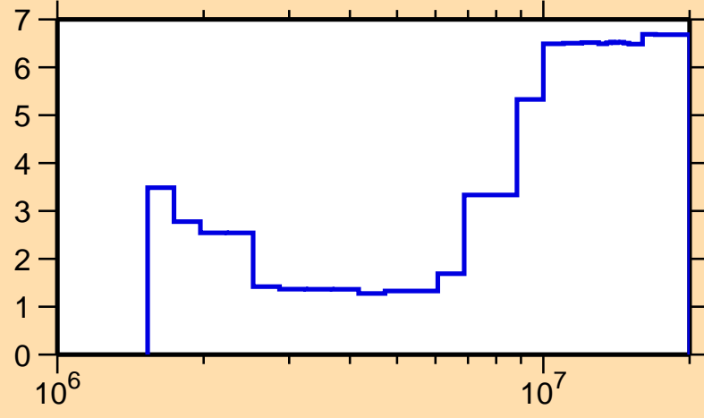
\Delta\sigma/\sigma vs. E for ^{162}\text{Dy}(n,\text{inel.})
