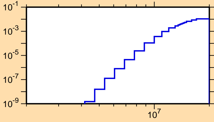
\sigma vs. E for ^{162}\text{Dy}(n,p)
