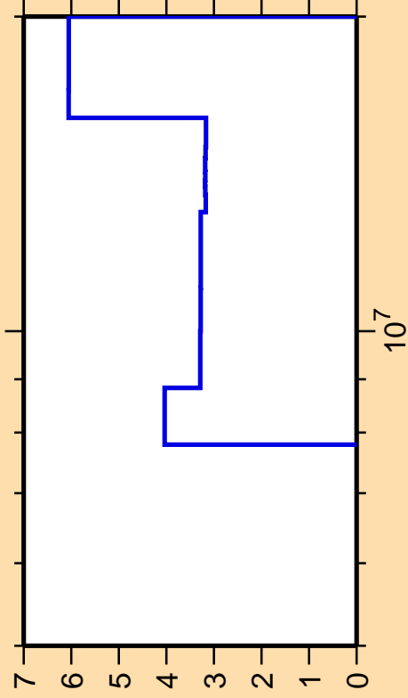
\Delta\sigma/\sigma vs. E for ^{162}\text{Dy}(n,2n)
