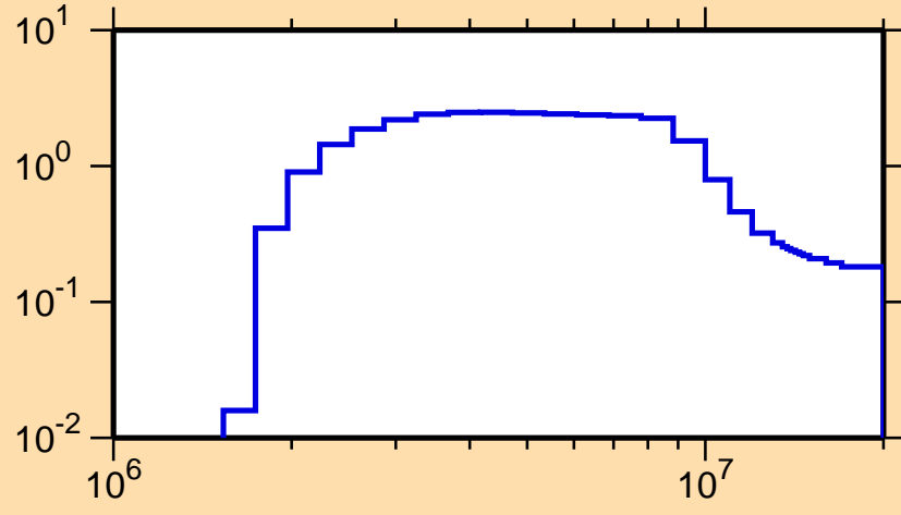
\sigma vs. E for ^{162}\text{Dy}(n,n\text{cont.})
