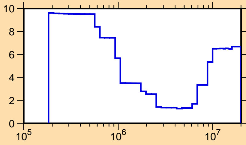
\Delta\sigma/\sigma vs. E for ^{162}\text{Dy}(n,\text{inel.})
