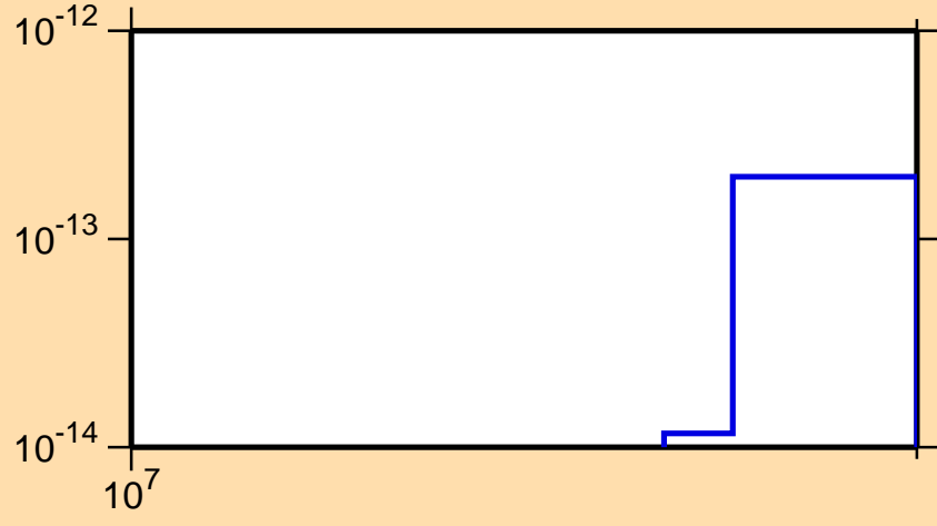
\sigma vs. E for ^{162}\text{Dy}(n,p\alpha)
