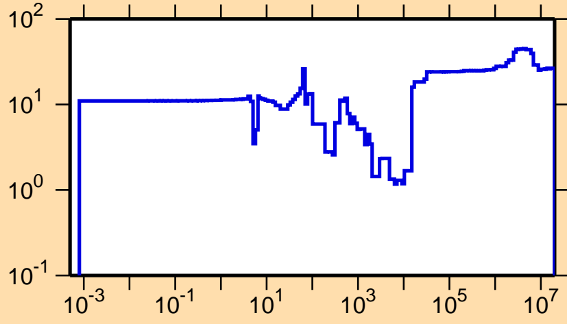
\Delta\sigma/\sigma vs. E for ^{162}\text{Dy}(n,\gamma)
