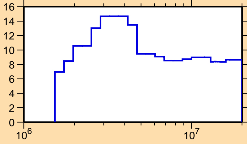
\Delta\sigma/\sigma vs. E for ^{162}\text{Dy}(n, n_1)
