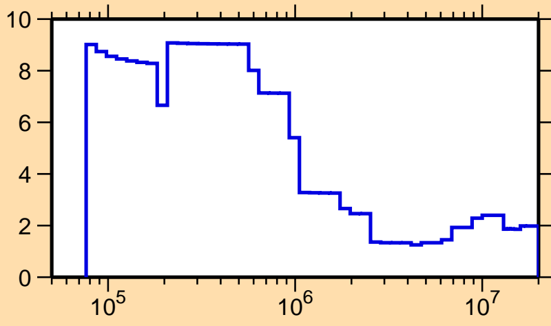
\Delta\sigma/\sigma vs. E for ^{162}\text{Dy}(n,\text{nonel.})
