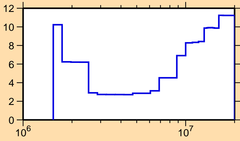
\Delta\sigma/\sigma vs. E for ^{162}\text{Dy}(n,n\text{cont.})
