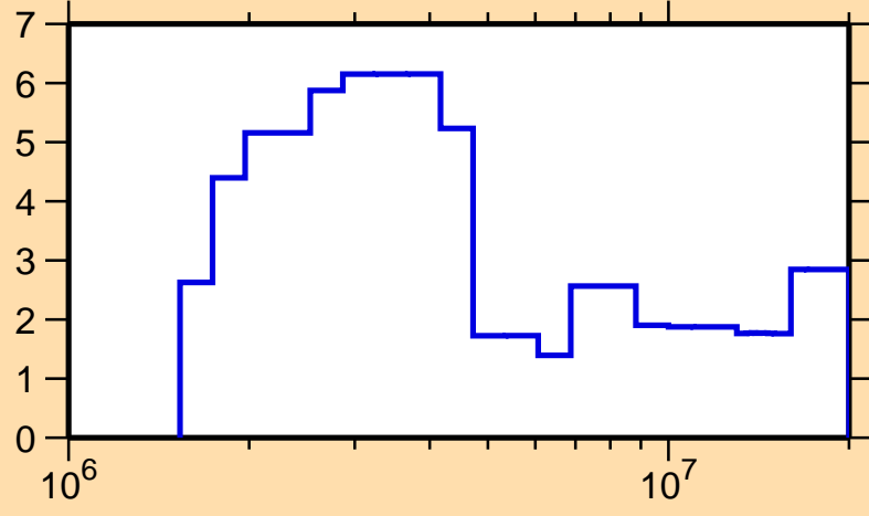
\Delta\sigma/\sigma vs. E for ^{162}\text{Dy}(n,el.)
