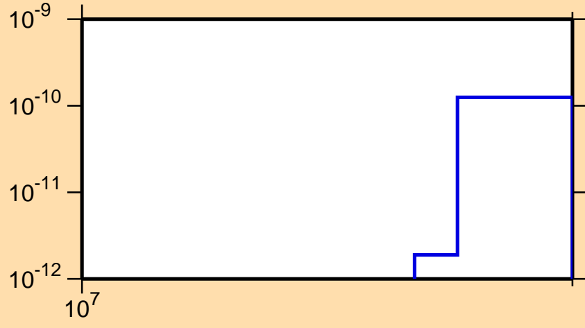
\sigma vs. E for ^{162}\text{Dy}(n,\text{He3})
