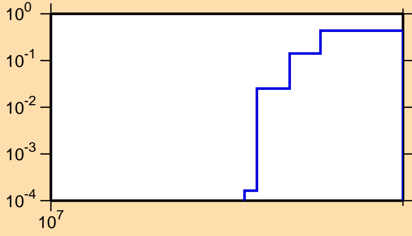
\sigma vs. E for ^{162}\text{Dy}(n,3n)
