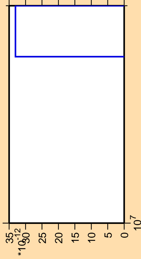
\Delta\sigma/\sigma vs. E for ^{162}\text{Dy} (mt 11)
