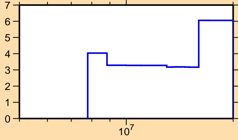
\Delta\sigma/\sigma vs. E for ^{162}\text{Dy}(n,2n)
