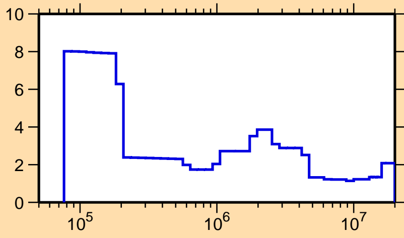
\Delta\sigma/\sigma vs. E for ^{162}\text{Dy}(n,\text{tot.})
