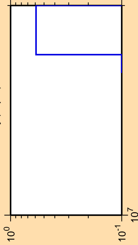
\Delta\sigma/\sigma vs. E for ^{162}\text{Dy}(n,p\alpha)
