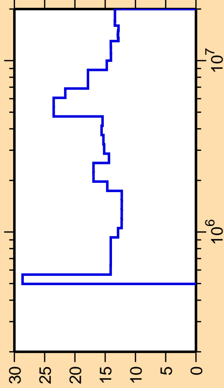
\Delta\sigma/\sigma vs. E for ^{162}\text{Dy}(n,n_3)
