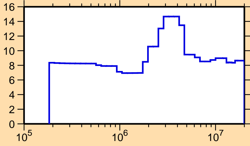
\Delta\sigma/\sigma vs. E for ^{162}\text{Dy}(n,n_1)
