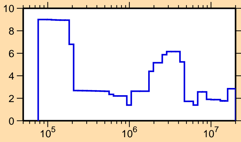
\Delta\sigma/\sigma vs. E for ^{162}\text{Dy}(n,\text{el.})
