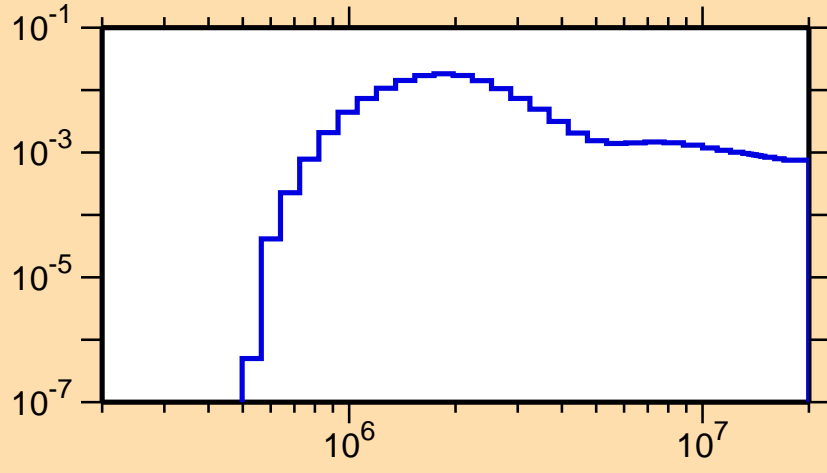
\sigma vs. E for ^{162}\text{Dy}(n,n_3)
