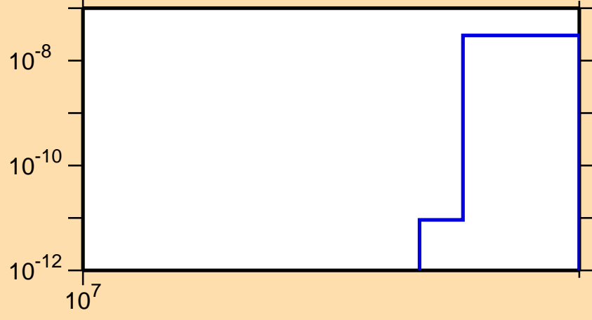
\sigma vs. E for ^{162}\text{Dy}(n,nd)
