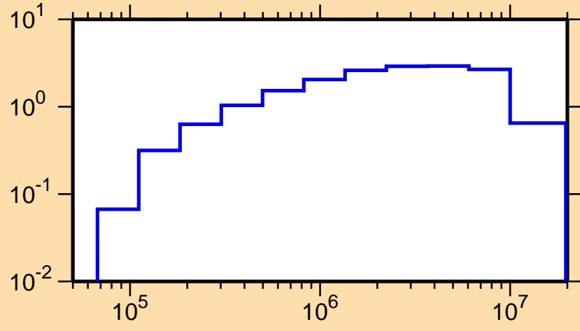
\sigma vs. E for ^{162}\text{Dy}(n,\text{inel.})
