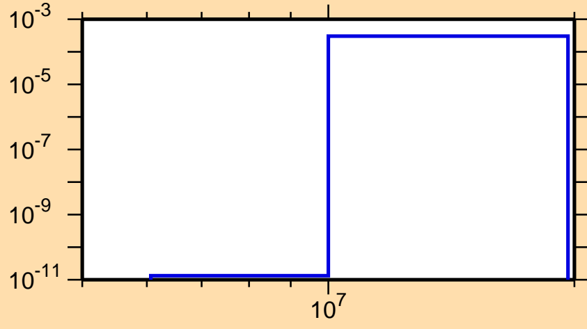
\sigma vs. E for ^{162}\text{Dy}(n,d)
