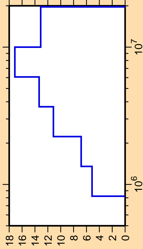
\Delta\sigma/\sigma vs. E for ^{162}\text{Dy}(n,n_4)
