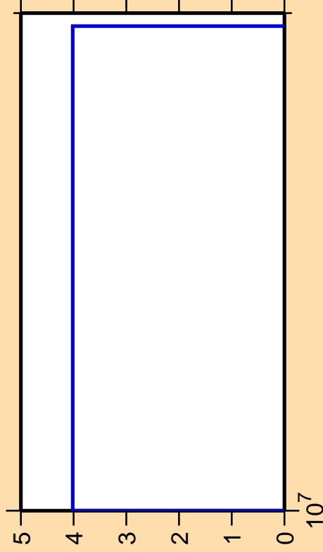
\Delta\sigma/\sigma vs. E for ^{162}\text{Dy}(n,\text{He}3)
