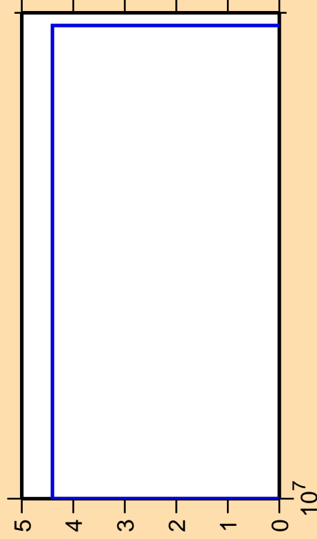
\Delta\sigma/\sigma vs. E for ^{162}\text{Dy}(n,3n)
