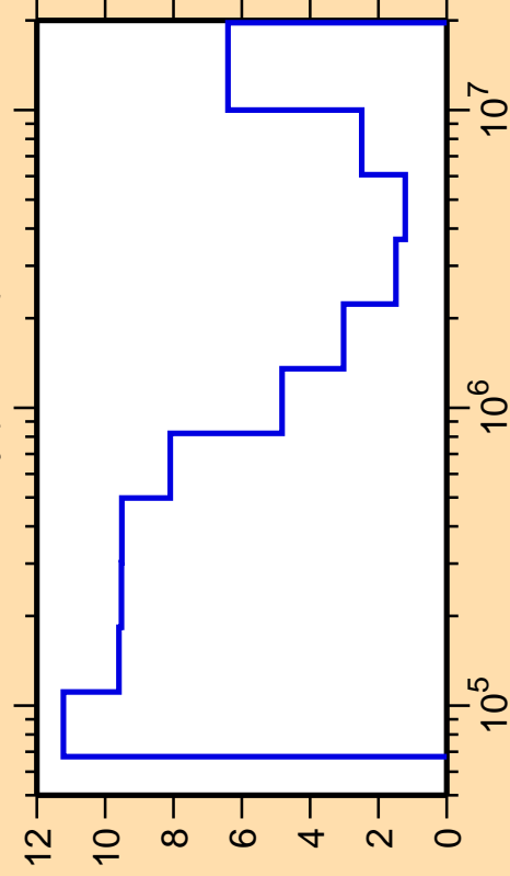
\Delta\sigma/\sigma vs. E for ^{162}\text{Dy}(n,\text{inel.})
