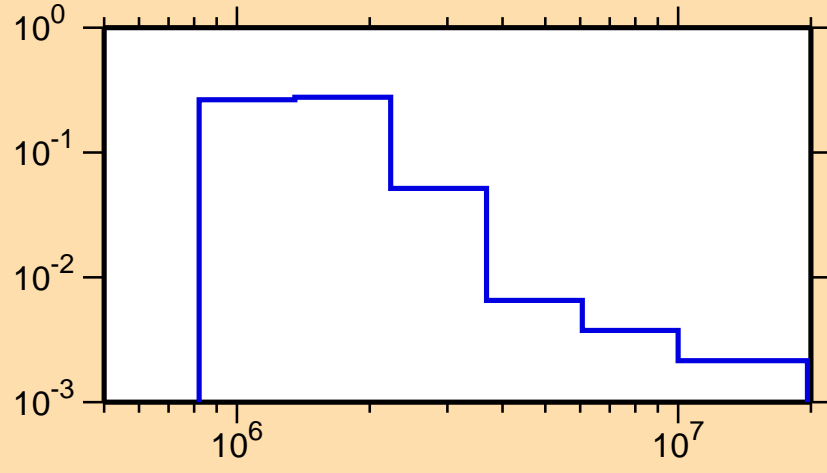
\sigma vs. E for ^{162}\text{Dy}(n,n_4)
