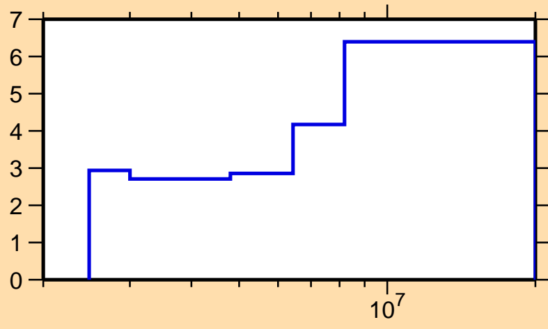
\Delta\sigma/\sigma vs. E for ^{162}\text{Dy}(n,n\text{cont.})
