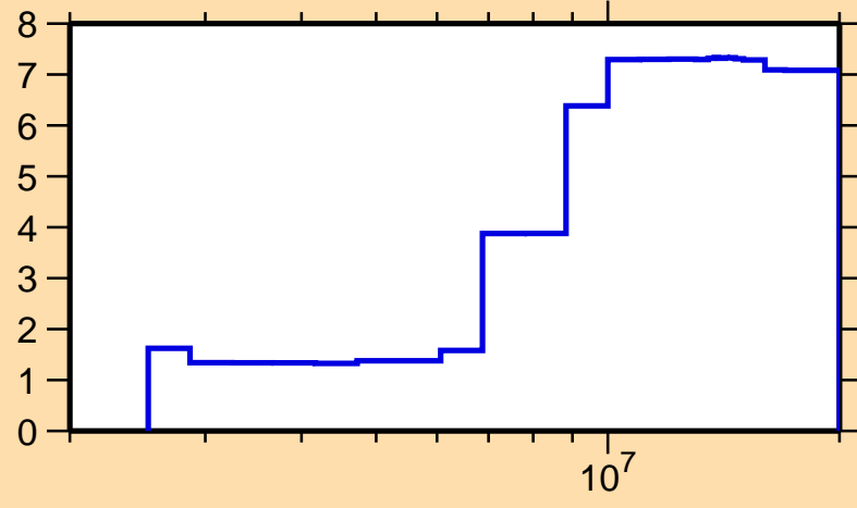
\Delta\sigma/\sigma vs. E for ^{163}\text{Dy}(n,\text{inel.})
