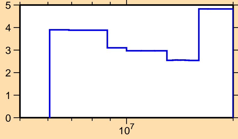
\Delta\sigma/\sigma vs. E for ^{163}\text{Dy}(n,2n)
