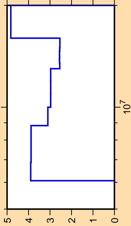
\Delta\sigma/\sigma vs. E for ^{163}\text{Dy}(n,2n)
