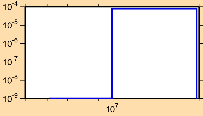
\sigma vs. E for ^{163}\text{Dy}(n,n\alpha)
