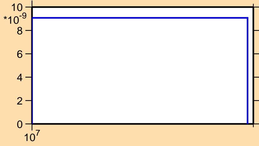
\sigma vs. E for ^{163}\text{Dy}(n,2n\alpha)
