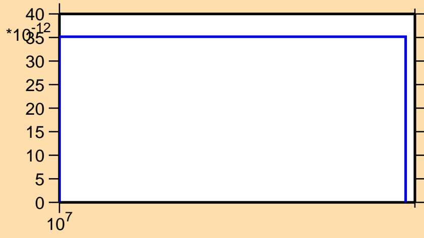
\sigma vs. E for ^{163}\text{Dy}(n,nt)
