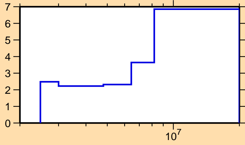
\Delta\sigma/\sigma vs. E for ^{163}\text{Dy}(n,n\text{cont.})
