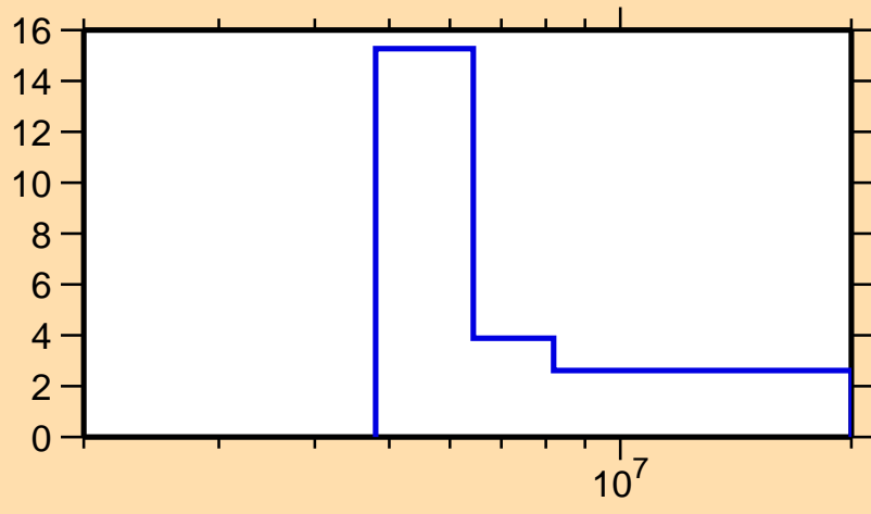
\Delta\sigma/\sigma vs. E for ^{163}\text{Dy}(n,2n)
