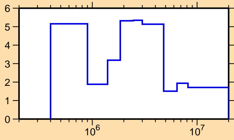
\Delta\sigma/\sigma vs. E for ^{163}\text{Dy}(n,el.)
