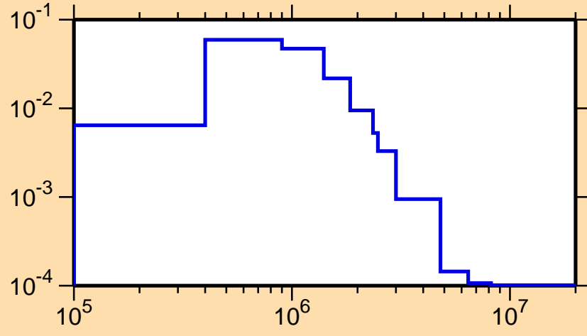
\sigma vs. E for ^{163}\text{Dy}(n,n_4)
