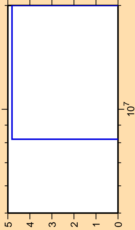
\Delta\sigma/\sigma vs. E for ^{163}\text{Dy}(n,3n)
