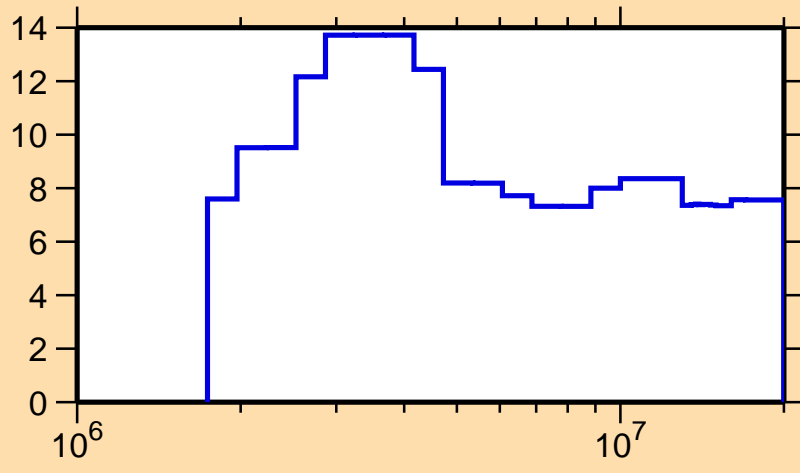
\Delta\sigma/\sigma vs. E for ^{164}\text{Dy}(n,n_1)
