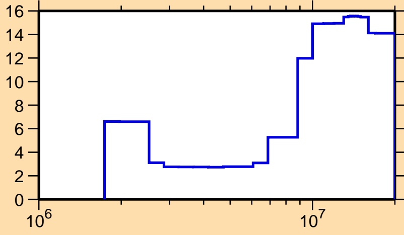
\Delta\sigma/\sigma vs. E for ^{164}\text{Dy}(n,n\text{cont.})
