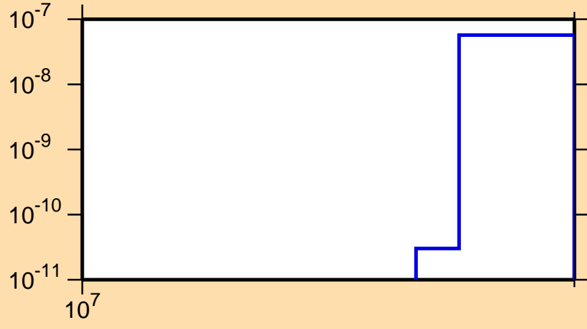
\sigma vs. E for ^{164}\text{Dy}(n,nd)
