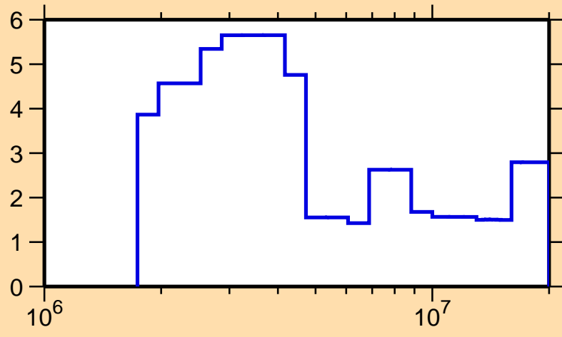
\Delta\sigma/\sigma vs. E for ^{164}\text{Dy}(n,el.)
