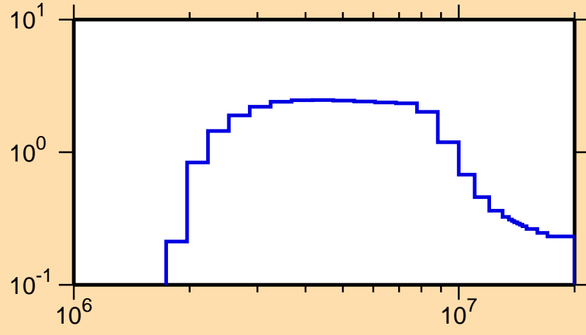
\sigma vs. E for ^{164}\text{Dy}(n,n\text{cont.})
