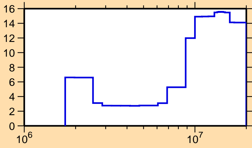
\Delta\sigma/\sigma vs. E for ^{164}\text{Dy}(n,n\text{cont.})
