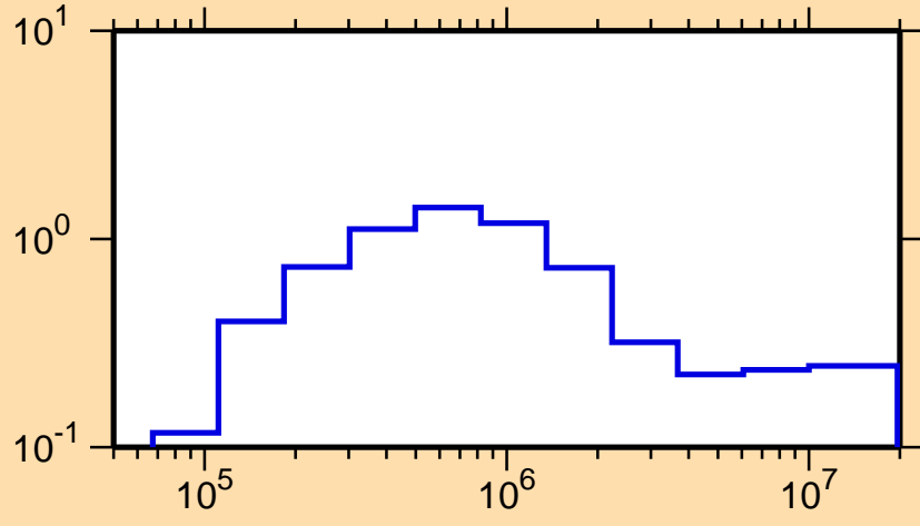
\sigma vs. E for ^{164}\text{Dy}(n,n_1)
