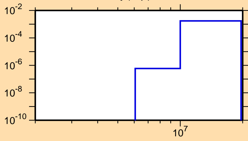
\sigma vs. E for ^{164}\text{Dy}(n,p)
