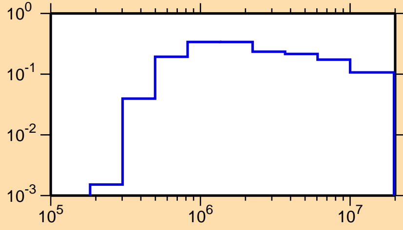
\sigma vs. E for ^{164}\text{Dy}(n,n_2)
