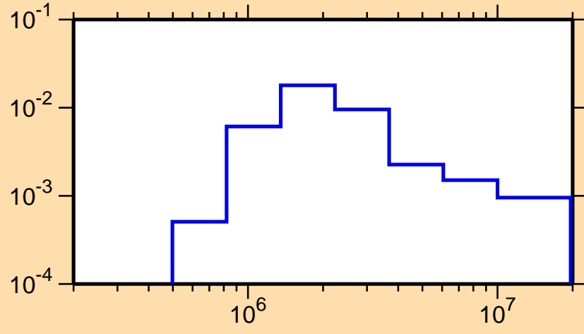
\sigma vs. E for ^{164}\text{Dy}(n,n_3)
