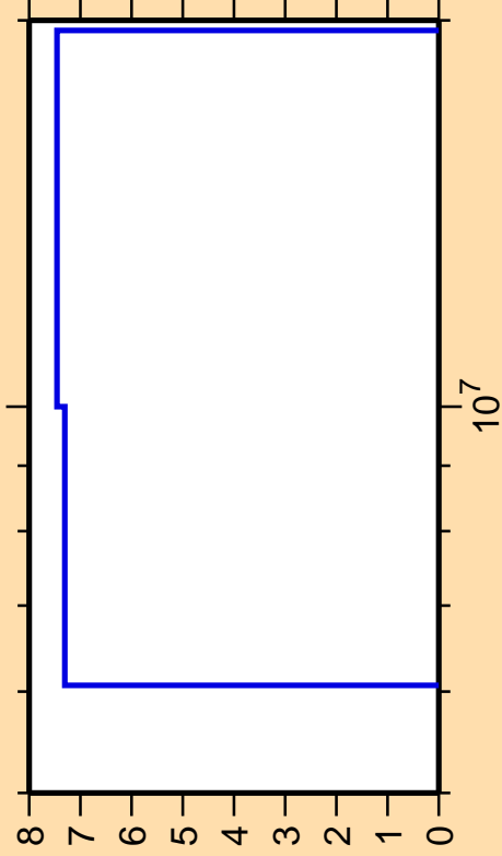
\Delta\sigma/\sigma vs. E for ^{164}\text{Dy}(n,n_1)
