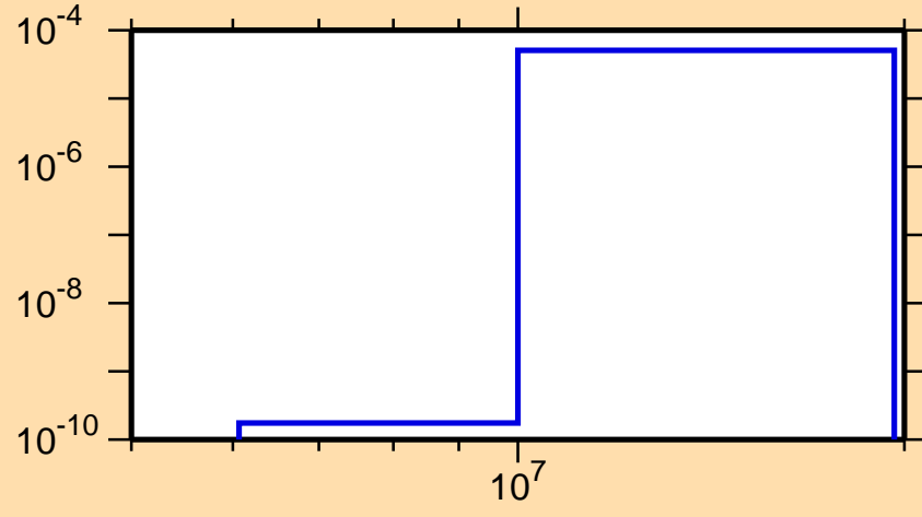
\sigma vs. E for ^{164}\text{Dy}(n,n\alpha)
