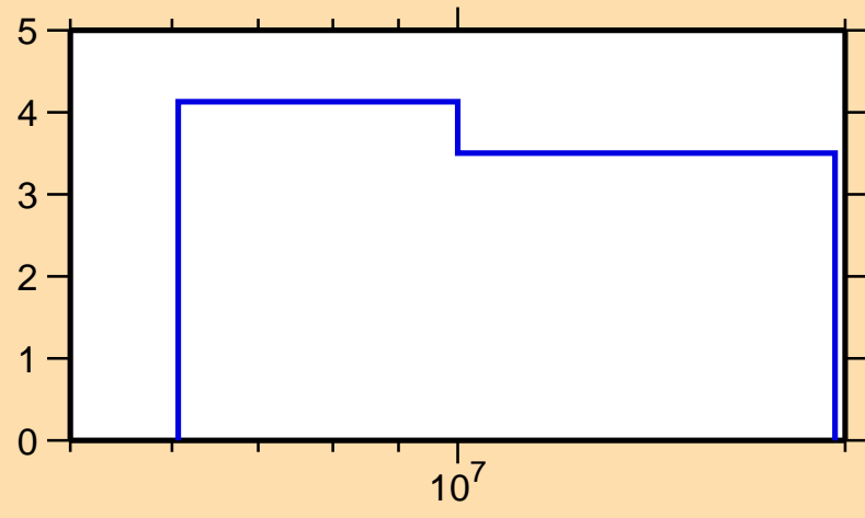
\Delta\sigma/\sigma vs. E for ^{164}\text{Dy}(n,2n)
