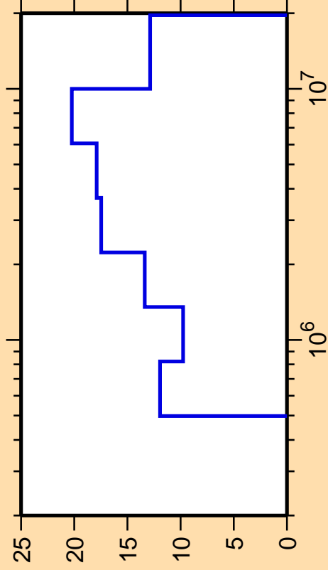
\Delta\sigma/\sigma vs. E for ^{164}\text{Dy}(n,n_3)
