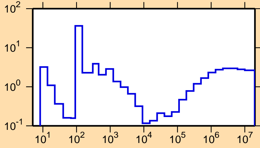
\sigma vs. E for ^{164}\text{Dy}(n,\text{nonel.})
