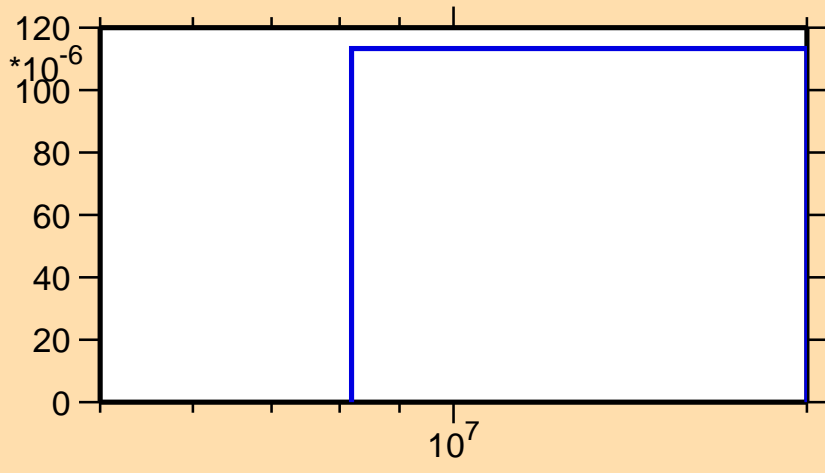
\sigma vs. E for ^{164}\text{Dy}(n,d)
