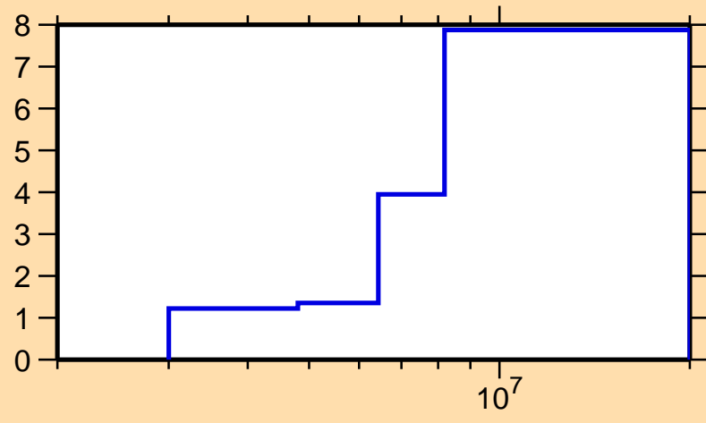
\Delta\sigma/\sigma vs. E for ^{164}\text{Dy}(n,\text{inel.})
