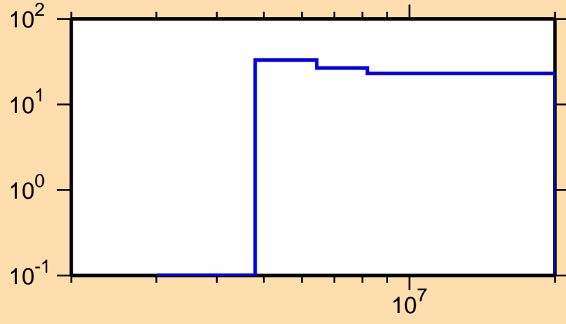
\Delta\sigma/\sigma vs. E for ^{164}\text{Dy}(n,p)
