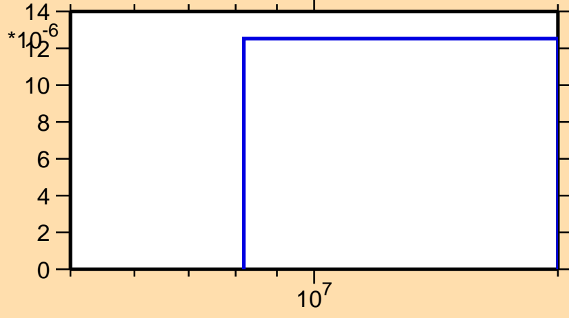
\sigma vs. E for ^{164}\text{Dy}(n,t)
