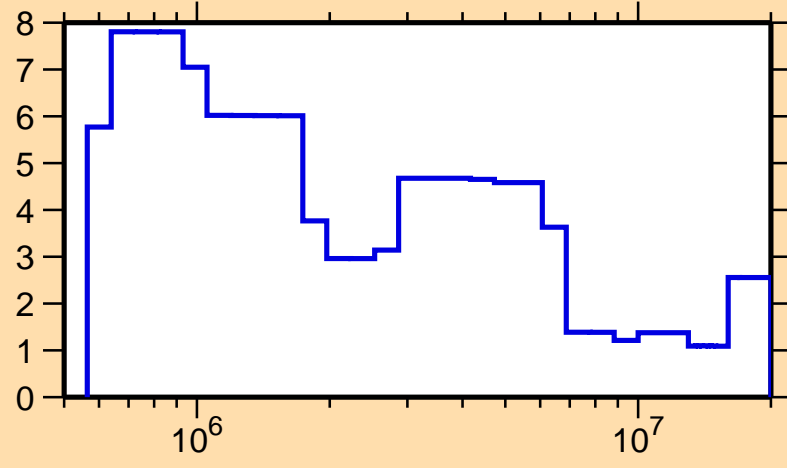
\Delta\sigma/\sigma vs. E for ^{165}\text{Dy}(n, tot.)
