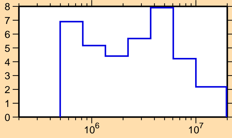
\Delta\sigma/\sigma vs. E for ^{165}\text{Dy}(n,el.)
