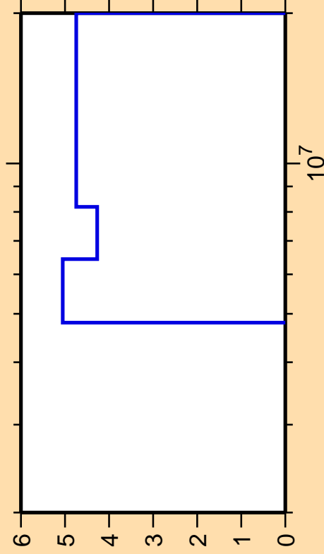
\Delta\sigma/\sigma vs. E for ^{165}\text{Dy}(n,2n)
