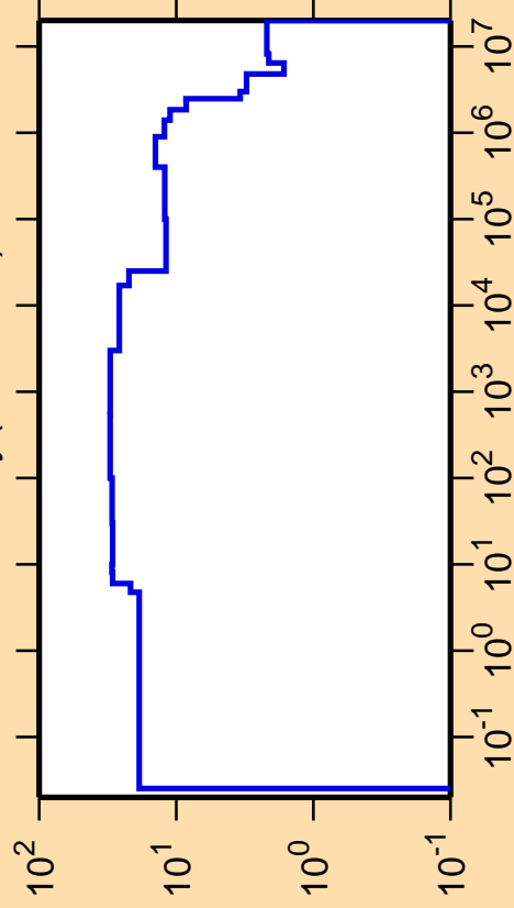
\Delta\sigma/\sigma vs. E for ^{165}\text{Dy}(n,\text{nonel.})
