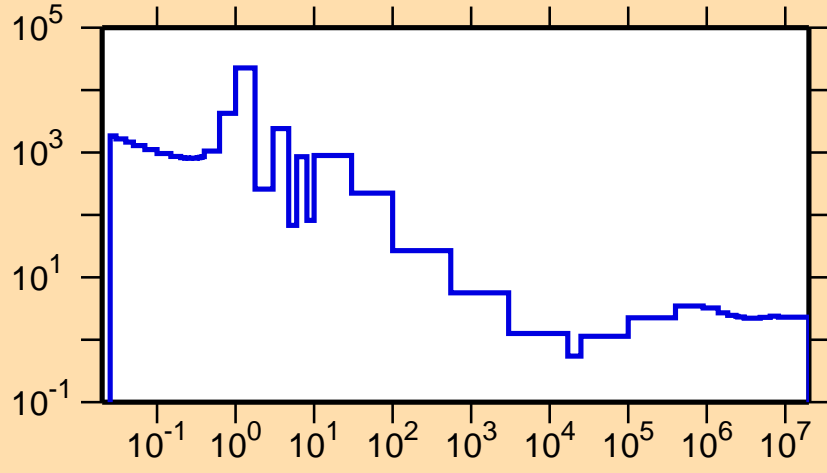
\sigma vs. E for ^{165}\text{Dy}(n,\text{nonel.})
