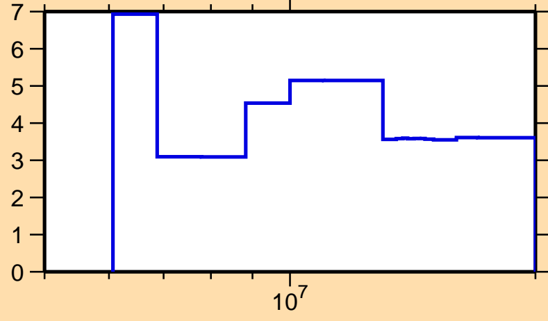
\Delta\sigma/\sigma vs. E for ^{166}\text{Dy}(n,\text{el.})
