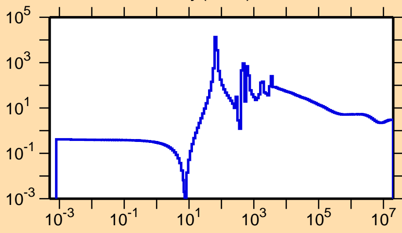
\sigma vs. E for ^{166}\text{Dy}(n,\text{el.})
