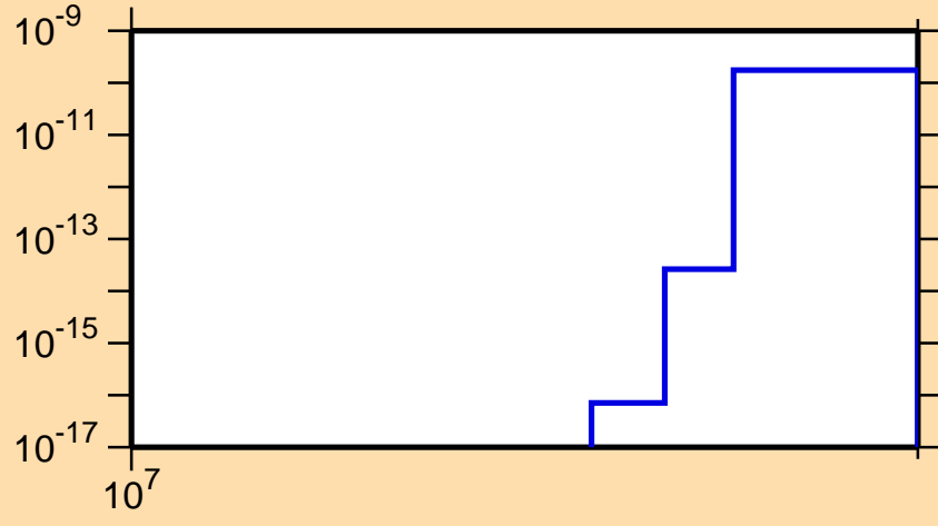
\sigma vs. E for ^{166}\text{Dy}(n,2np)
