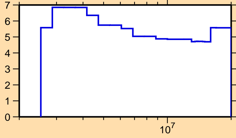
\Delta\sigma/\sigma vs. E for ^{166}\text{Dy}(n,\text{nonel.})
