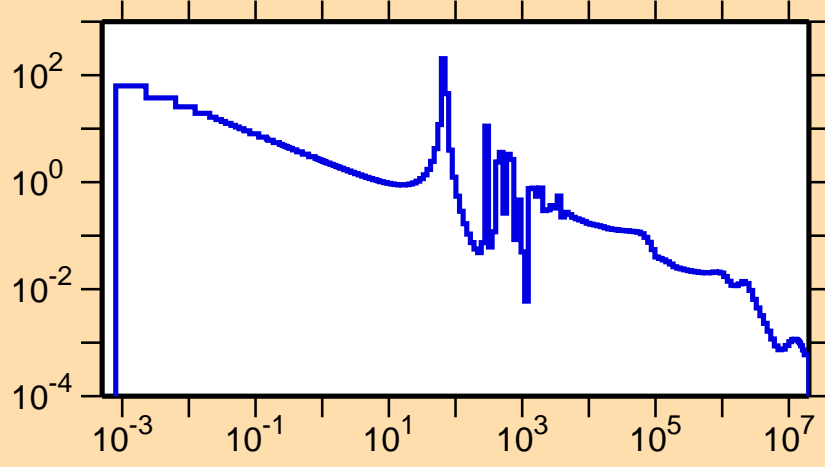
\sigma vs. E for ^{166}\text{Dy}(n,\gamma)
