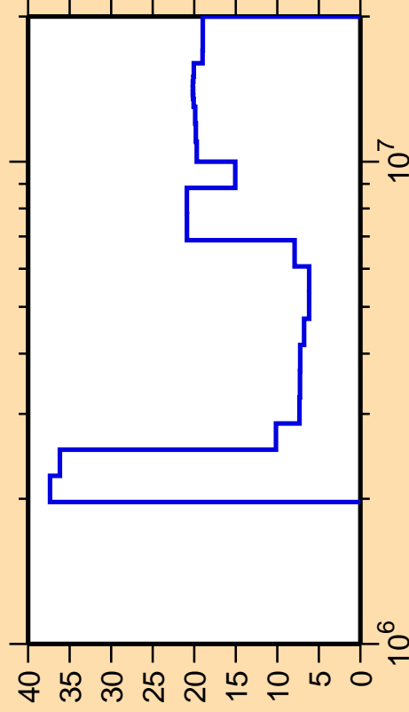
\Delta\sigma/\sigma vs. E for ^{166}\text{Dy}(n,n\text{cont.})
