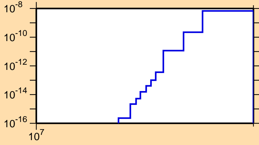
\sigma vs. E for ^{166}\text{Dy}(n,2n\alpha)
