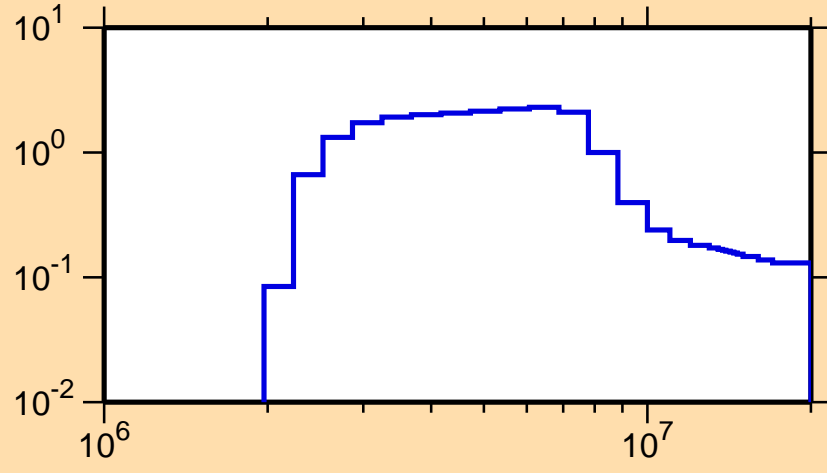
\sigma vs. E for ^{166}\text{Dy}(n,n\text{cont.})
